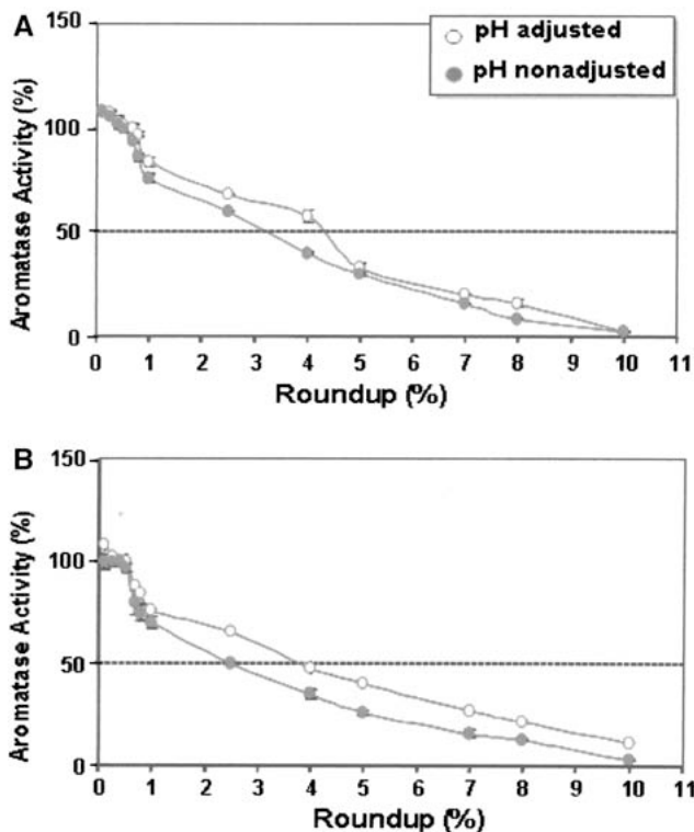
Fig. 5. Effects of Roundup on aromatase activity in human placental microsomes (A) and in equine testicular microsomes (B). The enzymatic activity was measured with pH nonadjusted decreasing to 4.88 at 10% (●) or pH adjusted to 7.4 (○) at 25°C after 15 min. The IC 50 is indicated by a dashed line
