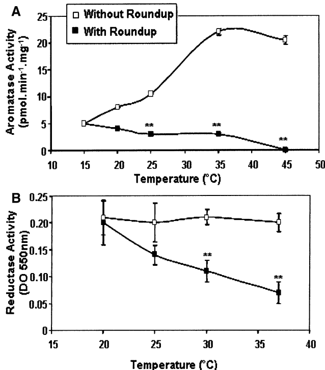
Fig. 6. Temperature influence on aromatase activity (A) and on reductase activity (B) in equine testicular microsomes or with the purified enzyme moiety, respectively. The enzymatic activity was measured in the absence (□) or in the presence of Roundup at IC 50 (■)
