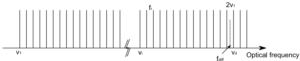
Fig. 10. Schematic spectrum of optical comb spanning one octave.
