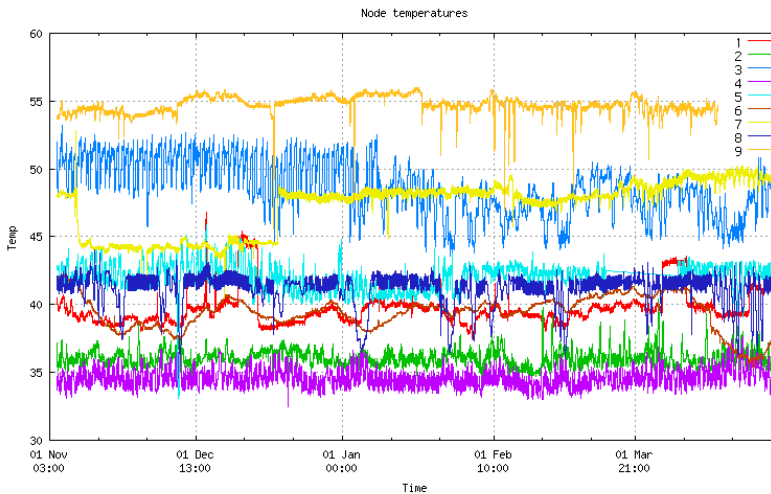
Fig. 2. Temperature measured in power supply in 9 telecom amplifier stations.
