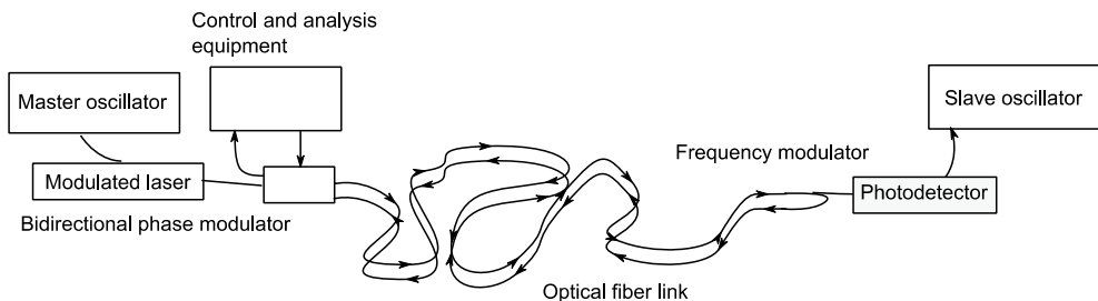
Fig. 9. Schematic frequency transfer in microwave domain.
