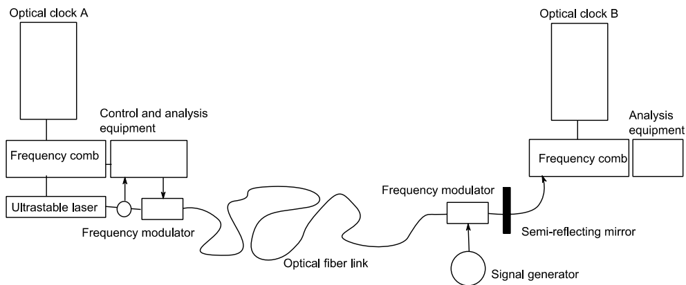
Fig. 11. Schematic setup for optical frequency transfer.
