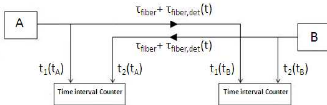
Fig. 3. Schematic system for two-way time transfer.
