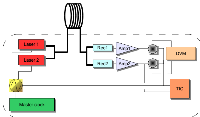
Fig. 7. Experimental setup. Rec1 and Rec2 include optical pre-amplification, optical band pass filter, photodiode and electrical trans-impedance amplifier. Amp1 and Amp2 are electrical amplifiers, DVM digital voltmeter and TIC is time-interval counter. Thin lines symbolize electrical wires and thick lines optical fibers.
