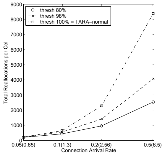
Fig. 13. Performance of reallocation minimisation algorithm. View (a)
