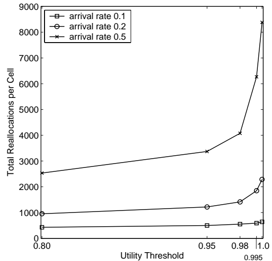
Fig. 14. Performance of reallocation minimisation algorithm. View (b)
