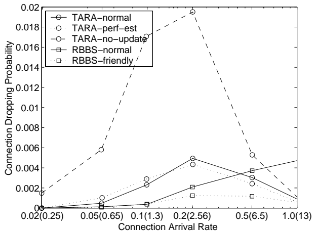
Fig. 10. Connection dropping probability
