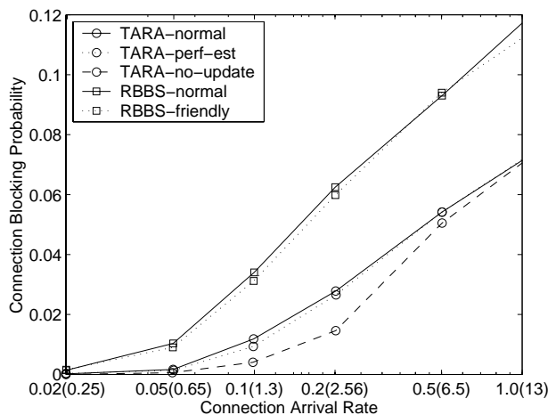
Fig. 9. Connection blocking probability
