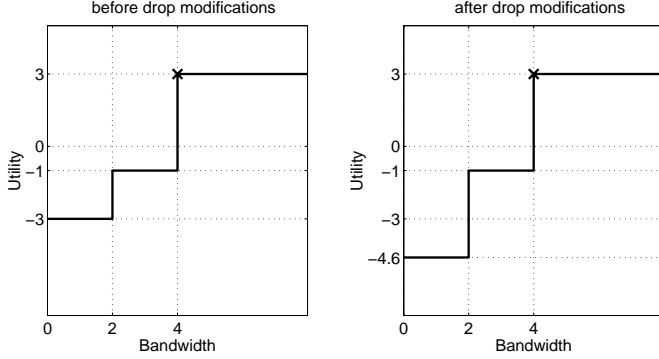
Fig. 4. Class II drop modification with P_i^{drop} = 8 , t_i^{age} = 5 , t_i^{max} = 10 , and actual bandwidth b_i = 4
