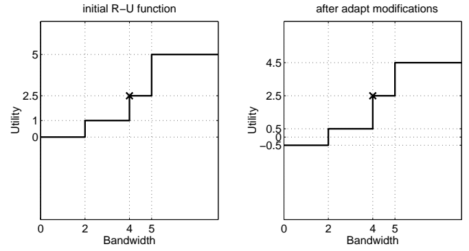
Fig. 5. Class III adaptation modification with A_i = 5 , I_i = 4 , P_i^{adapt} = 2 , and actual bandwidth b_i = 4
