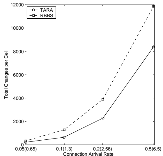
Fig. 11. Number of reallocations comparison
