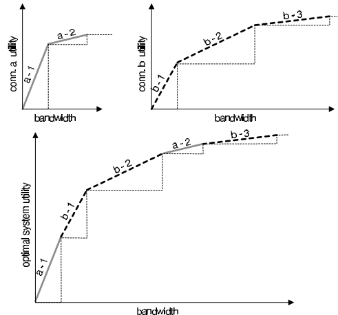
Fig. 1. Optimal allocation order
