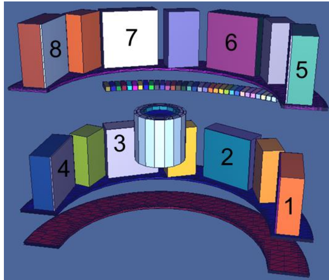
Figure 3. Simulation model.
