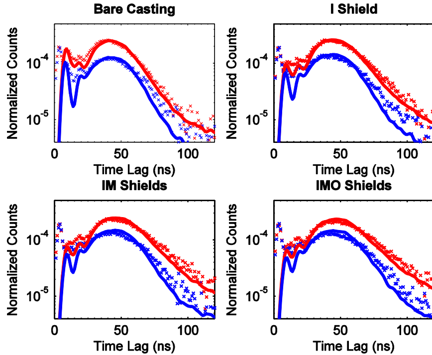
Figure 7. Comparison of simulations and measurements for all the shield combinations using detector #5 and pixel #11 of the \alpha detector. The solid lines are simulations, and the x's are measurements.
