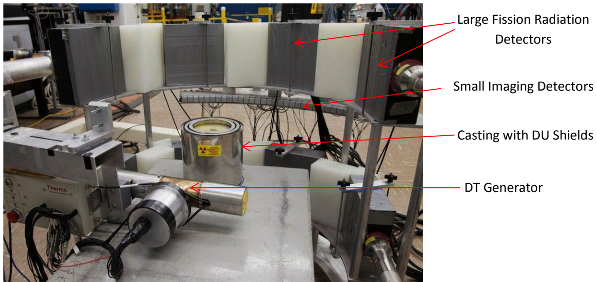
Figure 2. Arrangement of the detector system.
