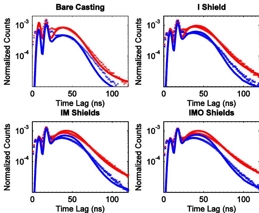
Figure 6. Comparison of simulations and measurements for all the shield combinations using the top row detectors and all pixels of the \alpha detector. The solid lines are simulations, and the x's are measurements.
