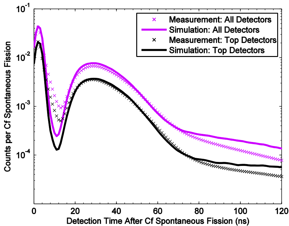
Figure 4. Comparison of the ^{252}\text{Cf} measurements and simulations.
