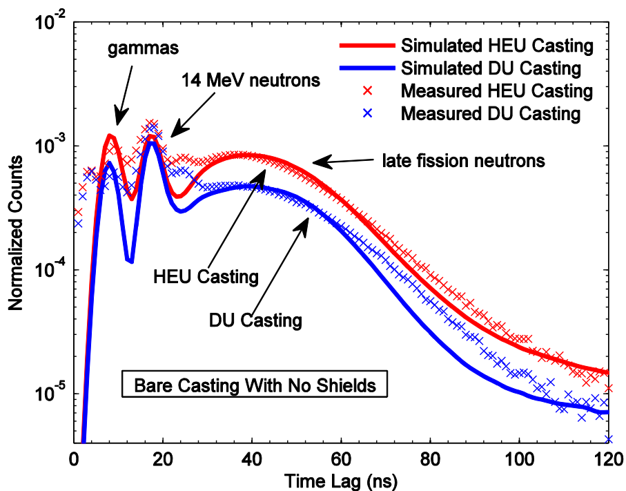
Figure 5. Comparison of the measurements and simulations for the bare castings.
