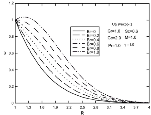
Fig. 18: Effect of Brinkman number ( Br ) on dimensionless temperature Profiles for time-dependent axial velocity of cylinder U(\tau) = \exp(-\tau)
