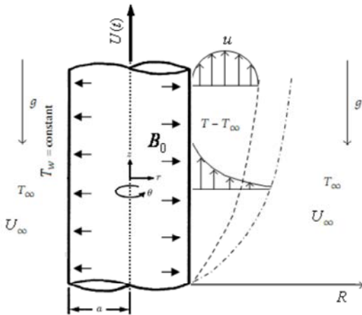
Fig. 1: Sketch of the physical model.
