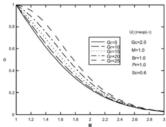
Fig. 3: Effect of Grashof number (Gr) on dimensionless temperature Profiles for \gamma = 0 and time-dependent axial velocity of cylinder U(\tau) = \exp(-\tau)
