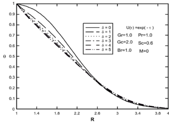
Fig. 16: Effect of thermal conductivity variation parameter ( \delta ) on dimensionless temperature Profiles for \gamma=0 and time-dependent axial velocity of cylinder U(\tau) = \exp(-\tau)
