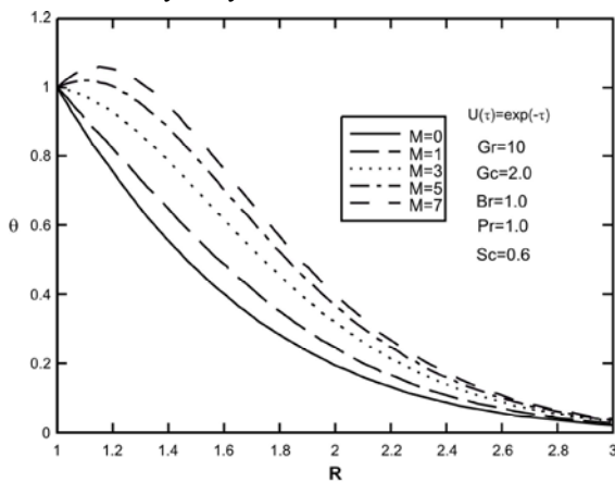
Fig. 6: Effect of magnetic parameter ( M ) on dimensionless temperature Profiles for \gamma = 0 and time-dependent axial velocity of cylinder U(\tau) = \exp(-\tau)
