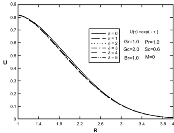
Fig. 15: Effect of thermal conductivity variation parameter ( \delta ) on dimensionless velocity Profiles for \gamma=0 and time-dependent axial velocity of cylinder U(\tau) = \exp(-\tau)
