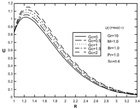
Fig. 4: Effect of mass Grashof number ( G_c ) on dimensionless velocity Profiles for \gamma = 0 and time-dependent axial velocity of cylinder U(\tau) = \exp(-\tau)
