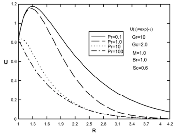
Fig. 7: Effect of Prandtl number on dimensionless velocity Profiles for \gamma = 0 and time-dependent axial velocity of cylinder U(\tau) = \exp(-\tau)
