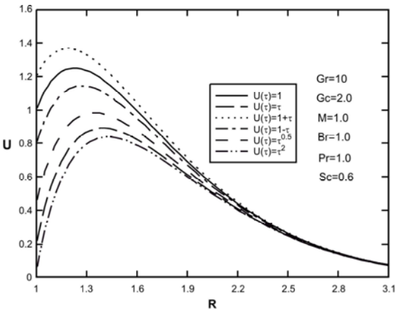
Fig. 11: Effect of different values time-dependent axial velocity of cylinder U(\tau) on dimensionless velocity Profiles for \gamma = 0
