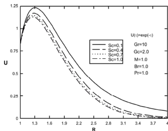
Fig. 9: Effect of Schmidt number ( Sc ) on dimensionless velocity Profiles for \gamma = 0 and time-dependent axial velocity of cylinder U(\tau) = \exp(-\tau)
