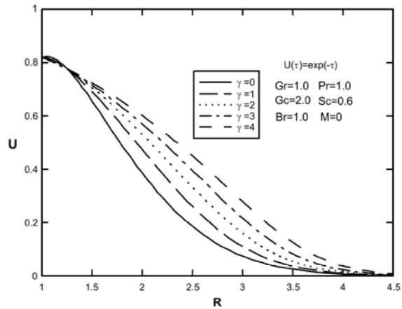
Fig. 13: Effect of viscosity-variation parameter ( \gamma ) on dimensionless velocity Profiles for time-dependent axial velocity of cylinder U(\tau) = \exp(-\tau)
