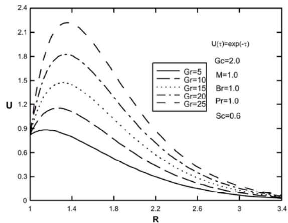
Fig. 2: Effect of Grashof number (Gr) on dimensionless velocity Profiles for \gamma = 0 and time-dependent axial velocity of cylinder U(\tau) = \exp(-\tau)
