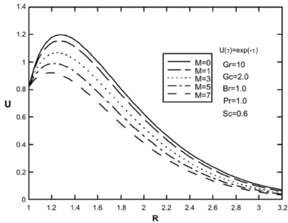
Fig. 5: Effect of magnetic parameter ( M ) on dimensionless velocity Profiles for \gamma = 0 and time-dependent axial velocity of cylinder U(\tau) = \exp(-\tau)
