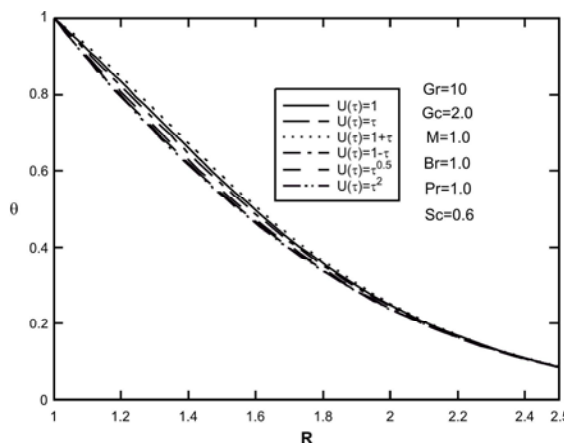
Fig. 12: Effect of different values time-dependent axial velocity of cylinder U(\tau) on dimensionless temperature Profiles for U(\tau) = \exp(-\tau)
