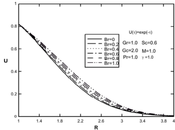
Fig. 17: Effect of Brinkman number ( Br ) on dimensionless velocity Profiles for time-dependent axial velocity of cylinder U(\tau) = \exp(-\tau)
