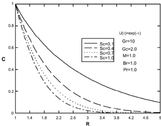
Fig. 10: Effect of Schmidt number ( Sc ) on dimensionless concentration Profiles for \gamma = 0 and time-dependent axial velocity of cylinder U(\tau) = \exp(-\tau)
