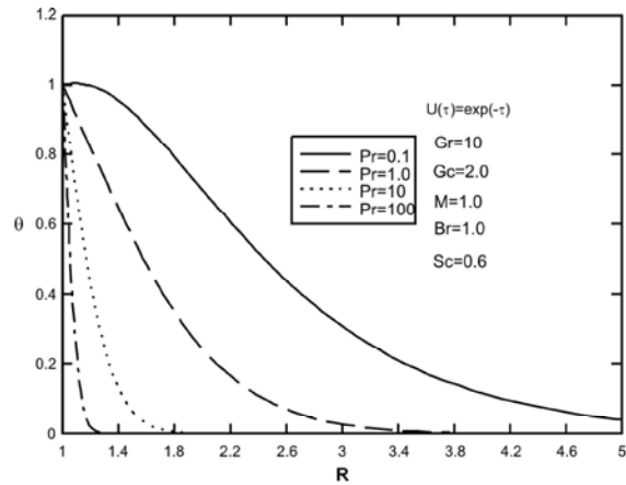
Fig. 8: Effect of Prandtl number on dimensionless temperature Profiles for \gamma = 0 and time-dependent axial velocity of cylinder U(\tau) = \exp(-\tau)
