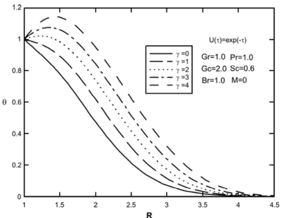
Fig. 14: Effect of viscosity-variation parameter ( \delta ) on dimensionless temperature Profiles for time-dependent axial velocity of cylinder U(\tau) = \exp(-\tau)
