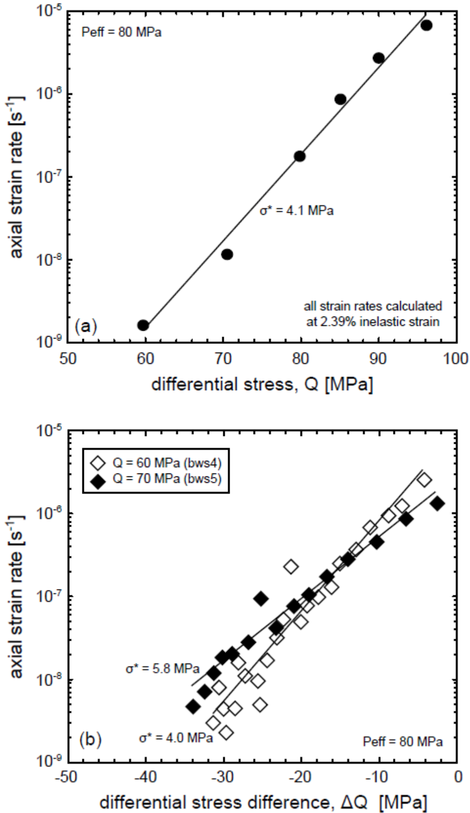
Figure 16. The stress-dependency of creep compaction. (a) Creep strain rates calculated at an inelastic strain of 2.39% for six creep experiments performed on Bleurswiler sandstone in
