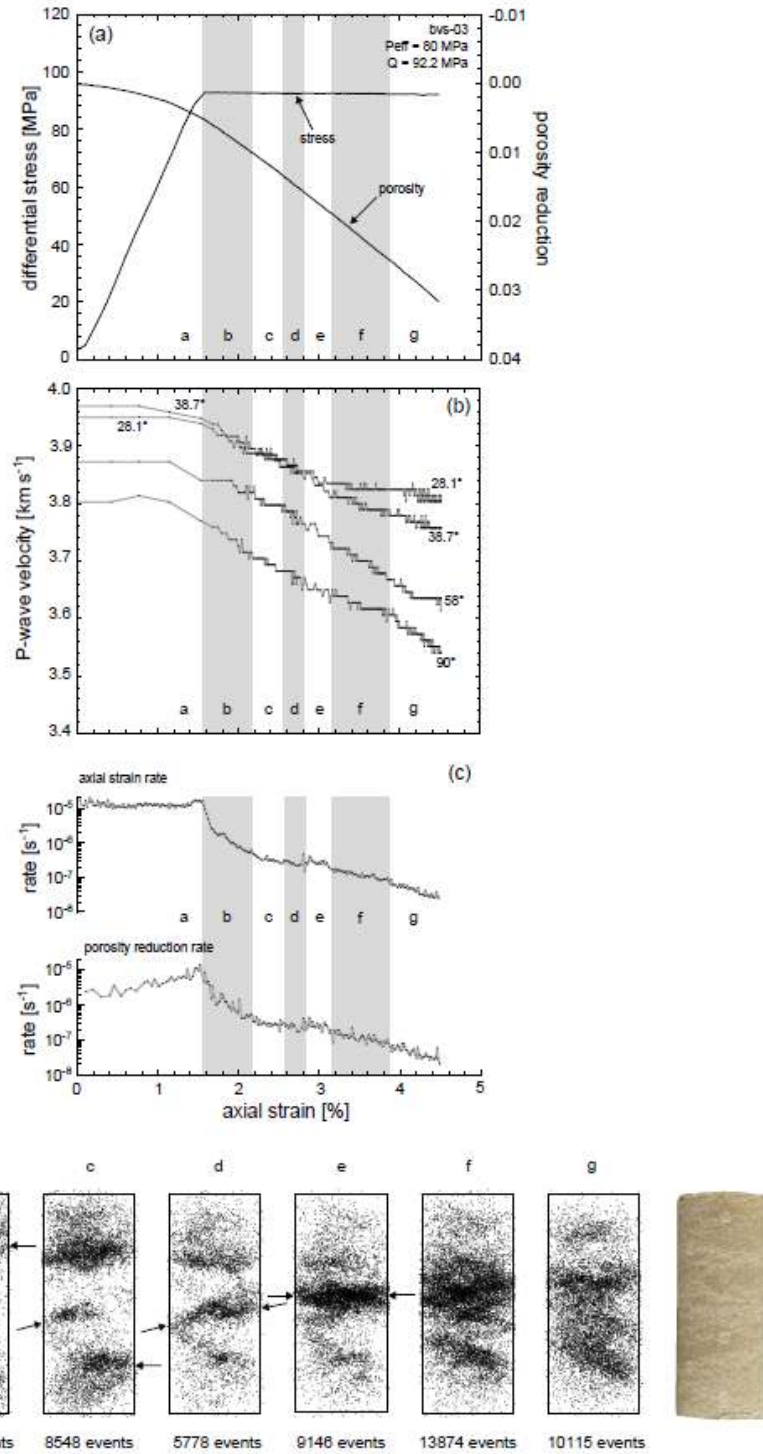
Figure 9. (a) Differential stress and porosity reduction as a function of axial strain for a constant stress ( Q = 92.2 \text{ MPa} ) experiment performed at an effective pressure of 80 \text{ MPa} on a sample of Bleurswiller sandstone. (b) The evolution of P-wave speeds during the experiment shown in panel (a). The angle corresponds to the angle of the propagation direction relative to the sample long axis. (c) Rates of axial strain and porosity reduction as a function of time for
