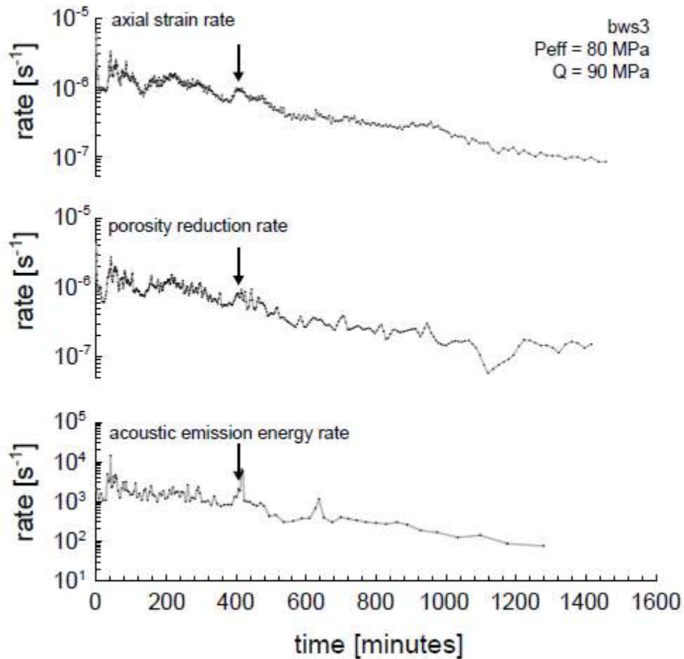
Figure 7. Rates of axial strain, porosity reduction, and acoustic emission energy against time ( t = 0 corresponds to the start of the constant stress portion of the experiment) for a constant stress experiment performed on a sample of Bleurswiller sandstone in the compactant regime (effective pressure = 80 MPa; creep stress = 90 MPa). The data presented here are for the experiment shown in Figures 6b and 6d. An example of a higher rate excursion has been indicated with arrows.
