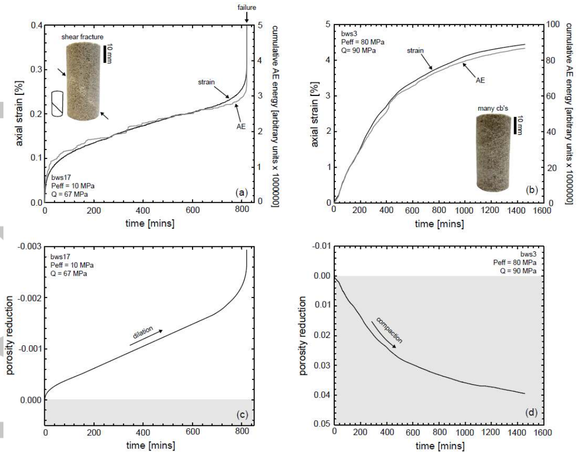
Figure 6. Blerswiller sandstone constant stress experiments. (a) Axial strain and accumulative acoustic emission energy as a function of time ( t = 0 corresponds to the start of the constant stress portion of the experiment) for a sample deformed in the dilatant regime (effective pressure = 10 MPa) at a constant stress of 67 MPa. Inset shows a photograph of the deformed sample and a schematic sample drawing highlighting the main features. (b) Axial strain and accumulative acoustic emission energy as a function of time ( t = 0 corresponds to the start of the constant stress portion of the experiment) for a sample deformed in the compactant regime (effective pressure = 80 MPa) at a constant stress of 90 MPa. Inset shows a photograph of the deformed sample; due to the density of compaction bands, the specific features are difficult to represent on a schematic sample drawing. (c) The porosity reduction curve for the dilatant experiment shown in panel (a). The grey zone denotes the area of net compaction. (d) The porosity reduction curve for the compactant experiment shown in panel
