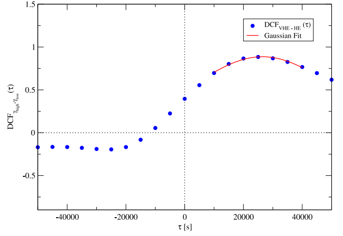
Figure 14. Discrete correlation function between the VHE \gamma -ray and HE \gamma -ray bandpasses for the proton spectral index perturbation. A positive lag indicates a HE \gamma -ray lag behind the VHE \gamma -rays.
