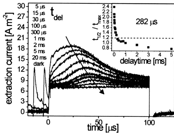
FIG. 3. Photo-CELIV transients recorded at 150 K at various delay times. The voltage rise speed A was 8 \text{ V}/100 \mu\text{s} . The inset shows the dispersion parameter t_{1/2} to t_{\text{max}} versus the delay time. The time to reach the ideal nondispersive value is also displayed.
