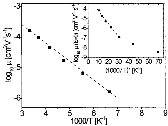
FIG. 10. Arrhenius plot of the mobility values taken at a constant E=5.2 \times 10^5 V cm ^{-1} electric field from Fig. 9. The inset shows the logarithm of mobility extrapolated to zero electric field versus (1000/T)^2 .
