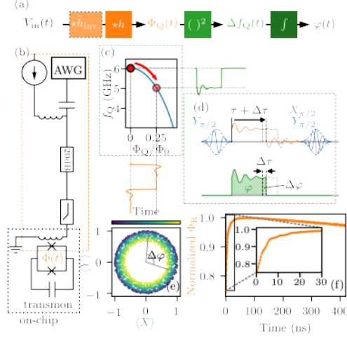
FIG. 1. Basic concept of Cryoscope. (a) Overview of relevant transformations involved. (b) Schematic of the control line used to control the flux \Phi_Q through the transmon SQUID loop. A DC source and AWG combined at a bias tee at room temperature produce the static and dynamic components of \Phi_Q . (c) When operating Cryoscope, the transmon is biased at its flux sweetspot and pulsed away only during the waiting interval between the \pi/2 pulses in a standard Ramsey-style experiment. (d) The difference in quantum phase \Delta\varphi [shown in (e)] acquired by the qubit during Ramsey experiments with the flux pulse truncated after \tau and \tau + \Delta\tau provides an estimate of the instantaneous qubit detuning \Delta f_Q in the interval [\tau, \tau + \Delta\tau] , and consequently an estimate \Phi_R of the instantaneous actual flux \Phi_Q . The nonlinear dependence of \Delta f_Q(\Phi_Q) suppresses the error produced by the difference of the two turn-off transients. (f) Reconstructed step response of the control line, normalized to maximal flux.
