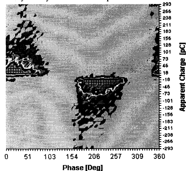
Fig. 5: Phase/height distributions of internal discharges at 17.8kV, 0.1Hz
