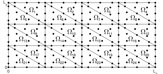
FIG. 1. An example of a mesh of a 2D rectangular domain, using triangular elements and having nodes for supporting P = 4 basis functions. The mesh is made up of N_{el} = 24 elements and contains 221 DOF's (nodes).
