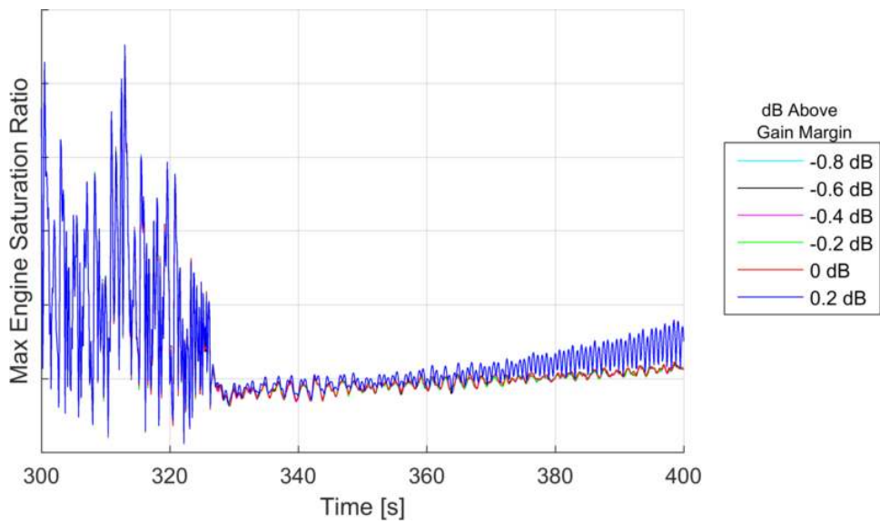
Figure 6: Max Engine Saturation Ratio for Rigid Body Gain Adjustments Applied at 300 Seconds
