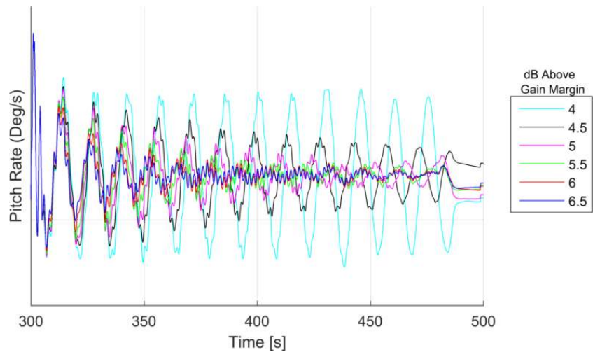
Figure 12: Aero Gain Instability at 300 Second with Regular Guidance.
