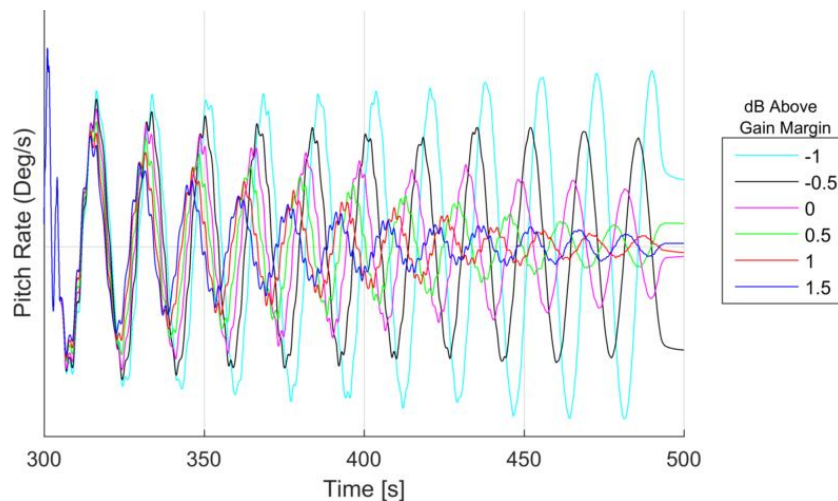
Figure 13: Aero Gain Instability at 300 Second with Frozen Guidance.
