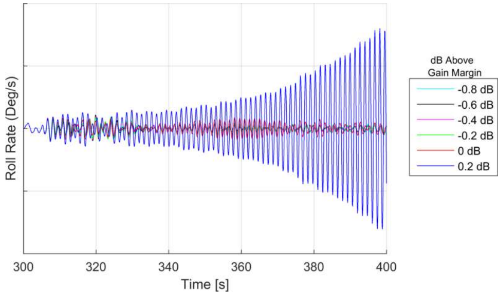
Figure 5: Roll Rate for Rigid Body Gain Adjustments Applied at 300 Seconds
