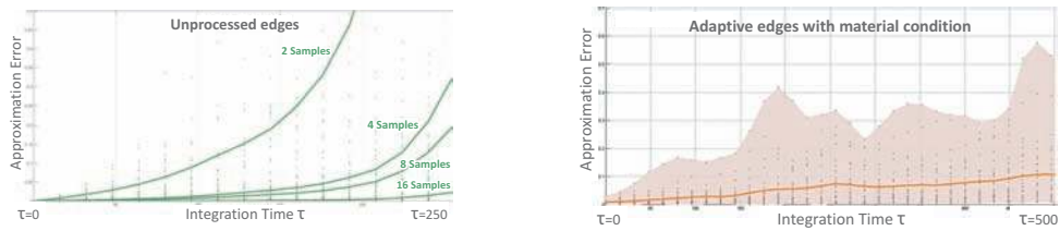
a) time line distance for 2, 4, 8, 16 samples b) time line distance of edges with material condition
