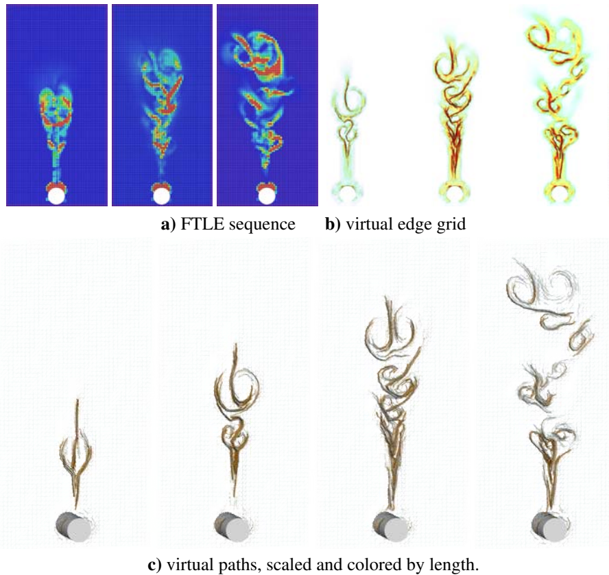
Abbildung 14: Heated Cylinder: Time sequence comparison for FTLE ( 60 \times 120 ) and triangulated virtual edge grid with 36 \times 72 and fixed \tau = 20 and t_0 = 20, 30, 40 .
