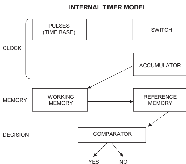
Fig. 1. Model of temporal information processing (redrawn from Church 1984).
