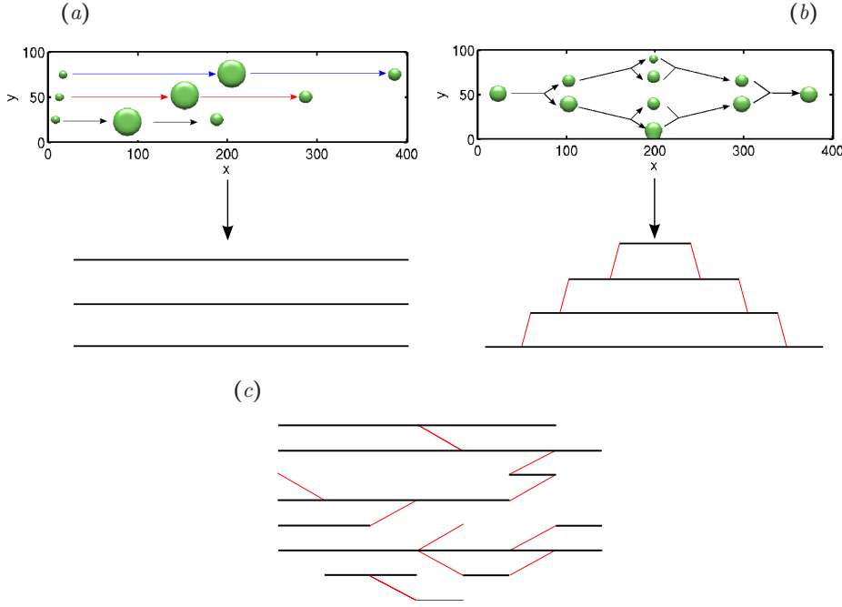
FIGURE 2. Artificially made test cases in arbitrary units. (a) Three objects moving with different advection velocities. (b) Objects splitting and merging. (c) Test with no physical meaning intended to check rare connections. For (a) and (b) the top figure shows the structures (in green) at different times (linked with arrows). The view is a x - y plane. The flow and time are going from left to right. The bottom part shows the corresponding graph with black lines for branches and red lines for mergers and splits. In case (c) only the graph is shown.
