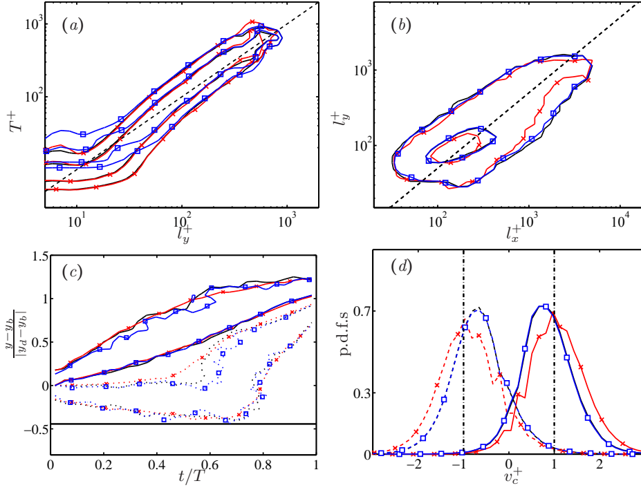
FIGURE 3. (a) P.d.f.s of the lifetimes of Q^- s primaries as a function of the wall-normal length of the branch, l_y . Each vertical section is a p.d.f. Contours are 40% and 80% of the maximum. The straight dashed line is T^+ = l_y^+ . (b) Joint p.d.f.s of the logarithm of the streamwise, l_x , and wall-normal, l_y , sizes of tall attached primaries. Data for ejections. The dashed straight line is l_x = 2l_y . Contours are 50% and 98% of the data. (c) P.d.f.s of the minimum (---) and maximum (—) heights of tall attached primary branches, as functions of the time elapsed from their birth. Time is normalized with the lifetime of each branch, T , and y_{min} and y_{max} with the heights, y_b and y_d , at its birth and death, respectively (see figure 10 in the paper). The solid horizontal lines are the average position of the wall. (d) P.d.f.s of the wall-normal velocity of the centre of gravity of sweeps (---) and ejections (—). The vertical dashed-dotted lines are v_c = \pm u_\tau . Symbols as in table 2.
