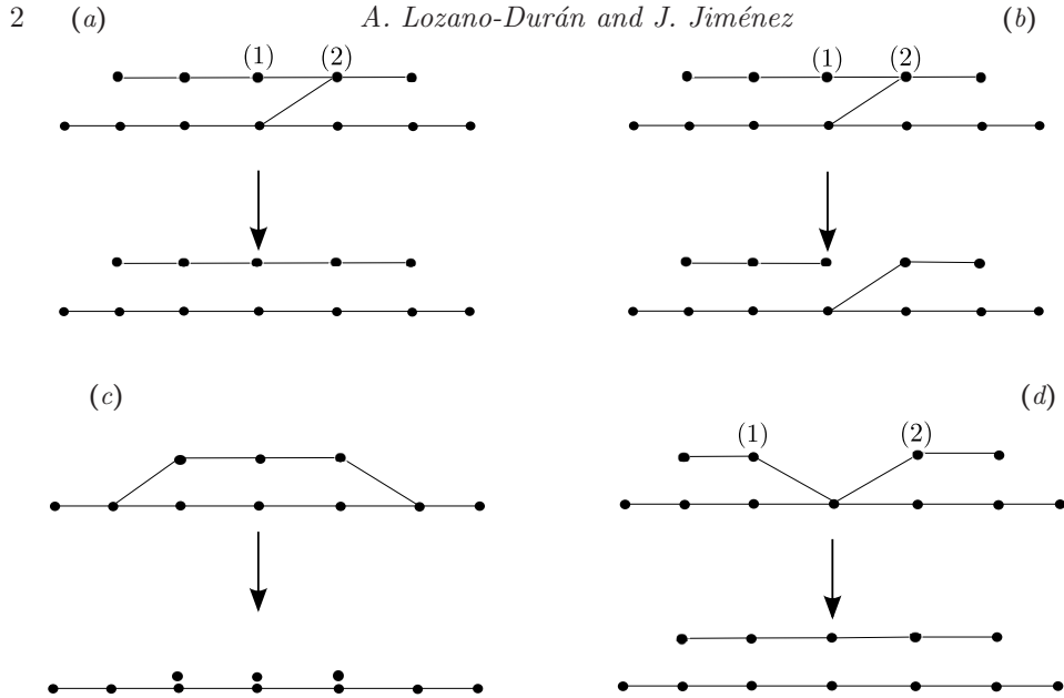
FIGURE 1. Sketches of the four types of connections corrected. For each graph, time is going from left to right. (a) Case I: two branches touch each other. The contact between them is dismissed. (b) Case II: two branches touch each other. One branch is disconnected in two. (c) Case III: a branch begins and ends at the same branch. Both of them are grouped into a single one. (d) Case IV: two branches are connected backward and forward with a third one at the same node. The two branches are disconnected and linked together to form a new one. See text for details of when the corrections are applied.
