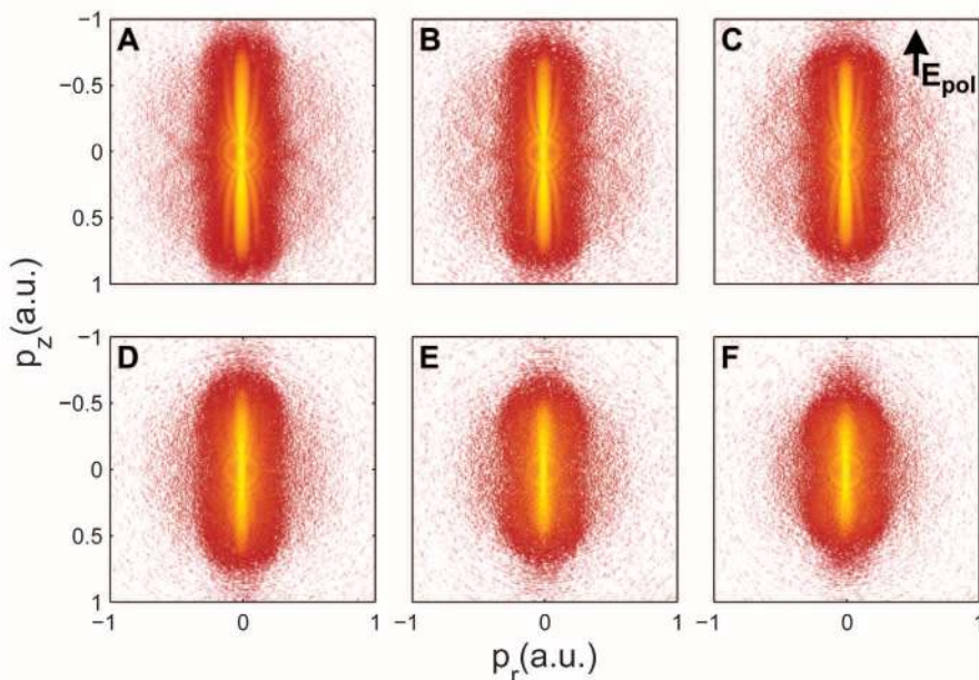
Fig. 2. Intensity dependence of measured velocity map images and the corresponding photoelectron kinetic energy distributions. (A) 7.1 \times 10^{11} \text{ W/cm}^2 ; (B) 5.5 \times 10^{11} \text{ W/cm}^2 ; (C) 4.5 \times 10^{11} \text{ W/cm}^2 ; (D) 3.2 \times 10^{11} \text{ W/cm}^2 ; (E) 2.5 \times 10^{11} \text{ W/cm}^2 ; and (F) 1.9 \times 10^{11} \text{ W/cm}^2 . (G) Angle-integrated photoelectron spectra. Squares indicate the energy that corresponds to the classical 2U_p cutoff energy.
