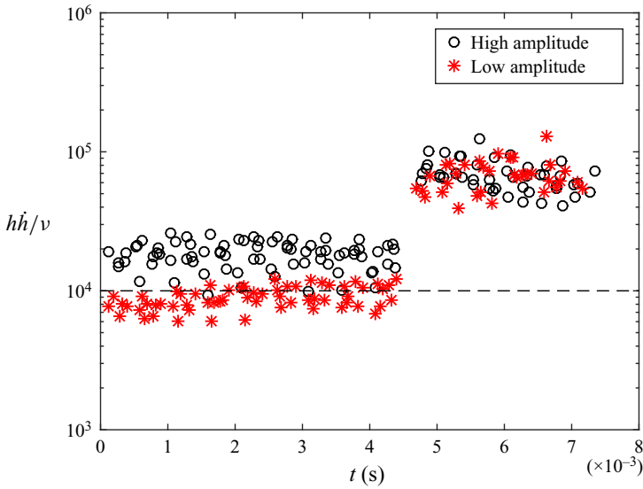
Figure 17. Outer-scale Reynolds number vs time for high- and low-amplitude experiments. The constant value of the Reynolds number is consistent for a growth exponent of \theta \approx 0.5 . The dashed black line indicates the Re = 10^4 threshold for mixing transition based on the criterion of Dimotakis (2000).
