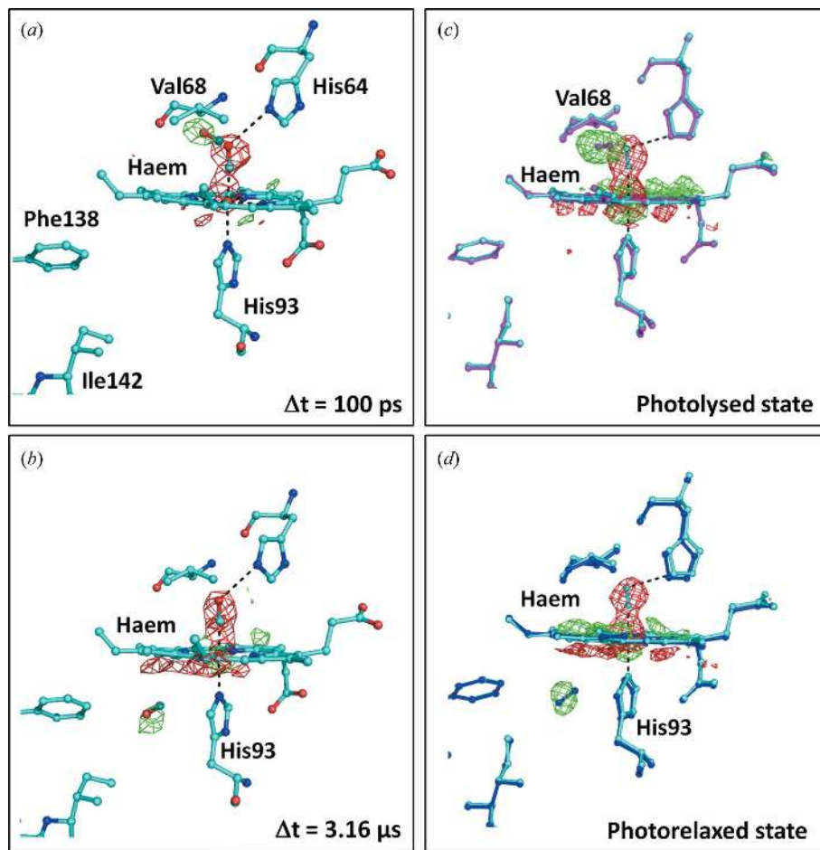
Figure 1 Time-resolved Laue diffraction and intermediate trapping studies of the photodissociation of carbon monoxide bound to the haem group of myoglobin. (a) F_{\text{obs}}(\text{light}) - F_{\text{obs}}(\text{dark}) difference Fourier electron density map of myoglobin (L29F) calculated for the time point 100 ps following photoactivation by a short laser pulse (Schotte et al. , 2003; Aranda et al. , 2006). Negative difference electron density (red) is observed 100 ps after photoactivation at the resting-state position of the carbon monoxide molecule (above the haem) and positive difference electron density (green) is observed nearby below Val68. (b) A similar map calculated for the time point 3.16 \mu s after photoactivation. At this time another binding pocket is visible as positive difference electron density (green) below the haem group near His93. In calculating these maps the crystallographic observations were taken from Protein Data Bank entries 2g0s (resting state), 2g0v (100 ps) and 2g14 (3.16 \mu s) (Aranda et al. , 2006). (c) Difference Fourier maps calculated from low-temperature trapping studies on wild-type myoglobin:carbon monoxide complexes (Chu et al. , 2000). The resting-state model is shown in cyan (Protein Data Bank entry 1dwr) and the photolysed state is shown in magenta (1dws). (d) Difference Fourier map calculated for the photorelaxed state, shown in blue (1dwt), from the same low-temperature study. All maps are contoured at 4.5\sigma . Agreement is apparent between the positions of the carbon monoxide molecule observed in the intermediate trapping and the Laue diffraction studies.
