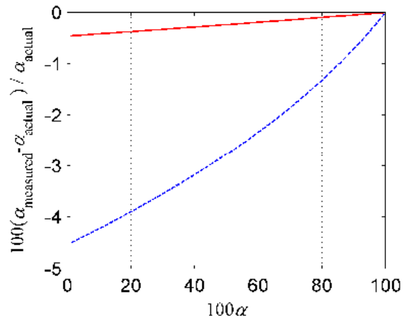
Fig. 4. The relative percent error in the measured void fraction versus the actual void fraction determined with equation 2, with a polychromatic beam and direct substitution of the detected light intensity, G , for number of photons at given energy, I(V) . The solid and dashed lines are for with and without pre-hardening, respectively.
