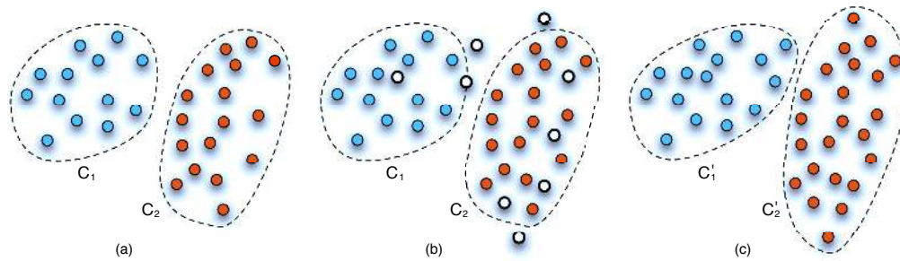
Fig. 3. The three main steps of a classification task. (a) A training set consisting of two pre-labeled classes C_1 and C_2 is entered into the system. The algorithm will first try to learn what the characteristic features distinguishing one class from another are; they are represented here by the class boundaries. (b) An unlabeled dataset is entered into the system that will then try to automatically deduce which class each datapoint belongs to. (c) Each point in the set entered has been assigned to a class. The system can then optionally adapt the classes boundaries.
