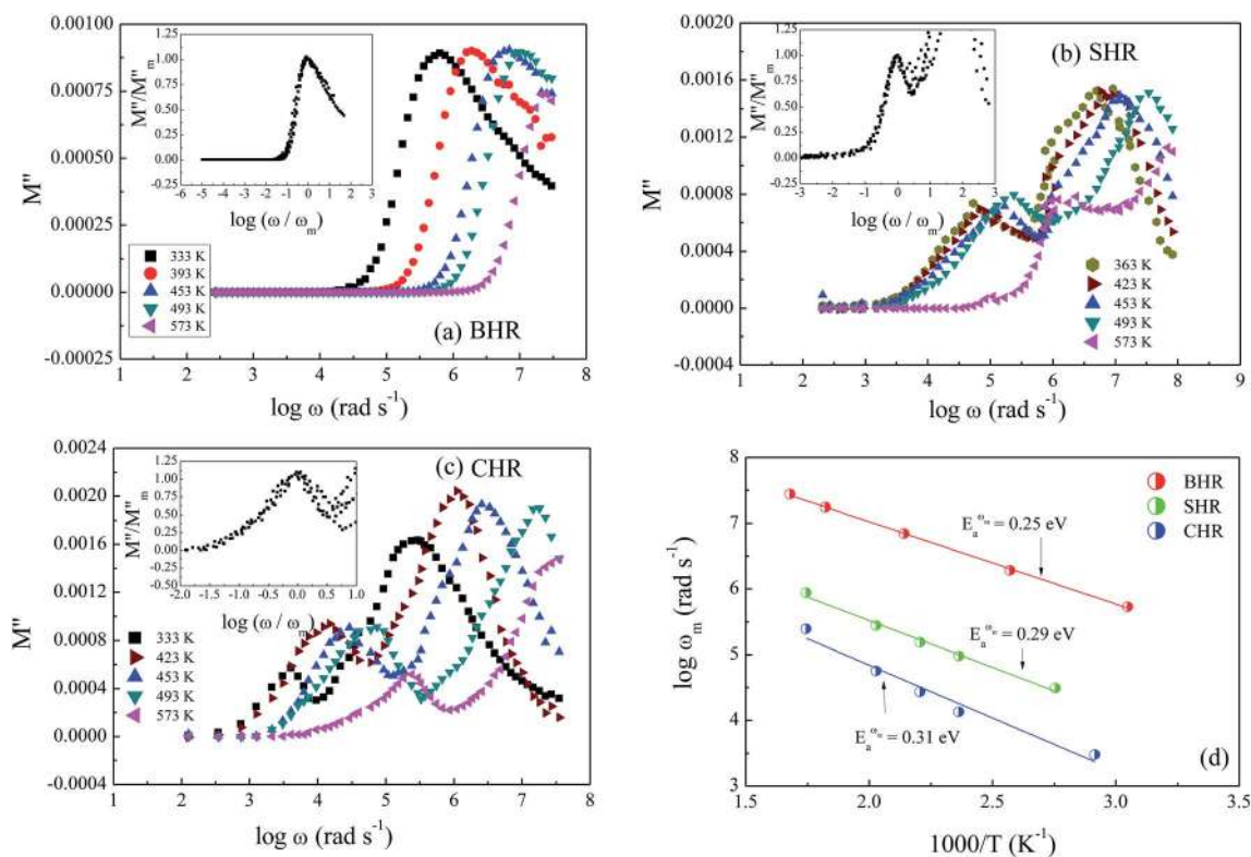
Fig. 10 Frequency dependent electric modulus ( M'' ) for (a) \text{Ba}_2\text{HoRuO}_6 (BHR), (b) \text{Sr}_2\text{HoRuO}_6 (SHR) and (c) \text{Ca}_2\text{HoRuO}_6 (CHR). The insets show the scaling behaviour. (d) Thermal variation of relaxation frequency ( \omega_m ) for BHR, SHR and CHR.
