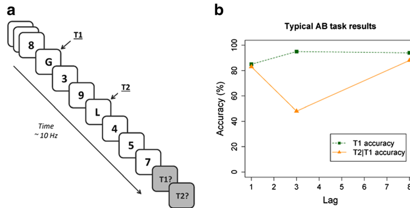
Fig. 1 a) The design and b) the results of a typical AB task
