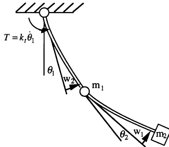
Figure 2.3.2 Two Link Model with Rate Command
