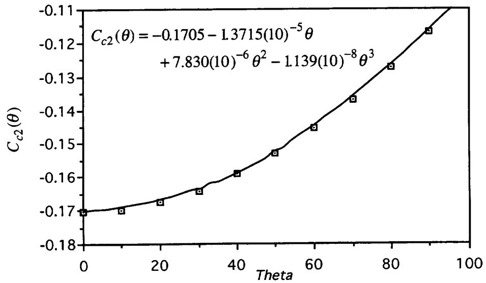
Figure 4.6.10 SVO Compensator Parameter C_{c2}(\theta)
