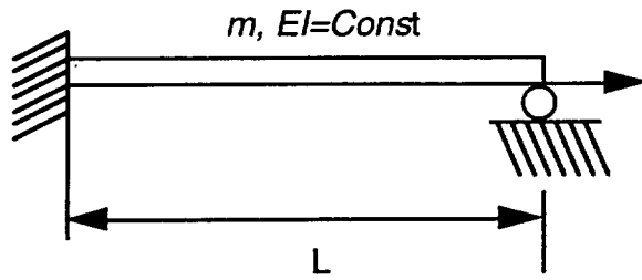
Figure 2.4.1 Cantilever Hinged Problem
