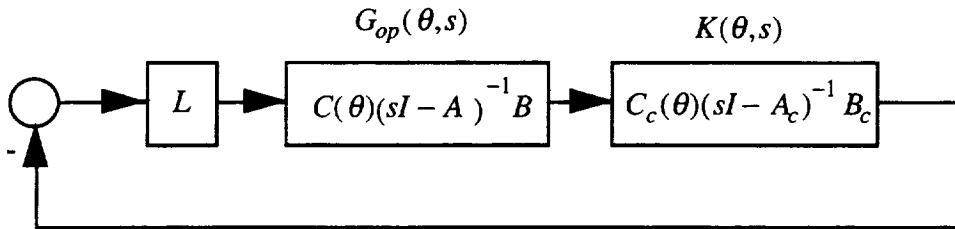
Figure 4.4.2 Diagonal Gain and Phase Change Matrix at Plant Input
