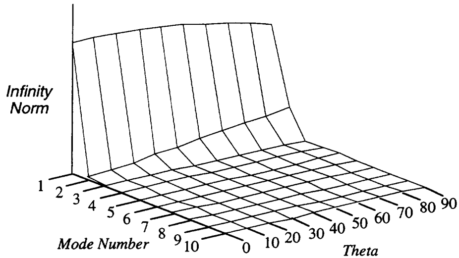
Figure 2.6.1 Infinity Norm of Bode Response as a Function of Mode Number and Theta - Heavy Payload
