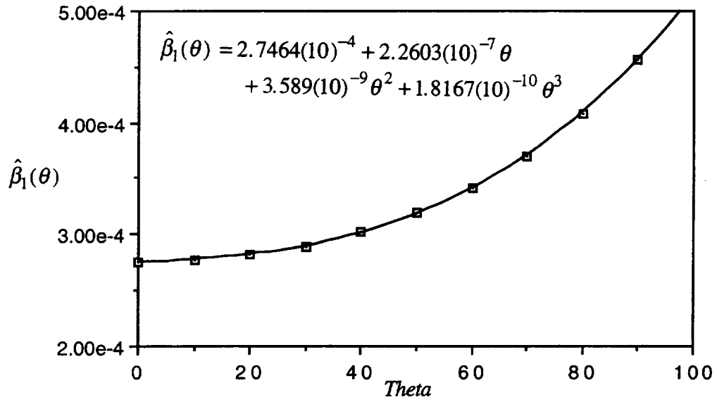
Figure 3.5.1 Identified Polynomial \hat{\beta}_1(\theta) as Function of Theta
