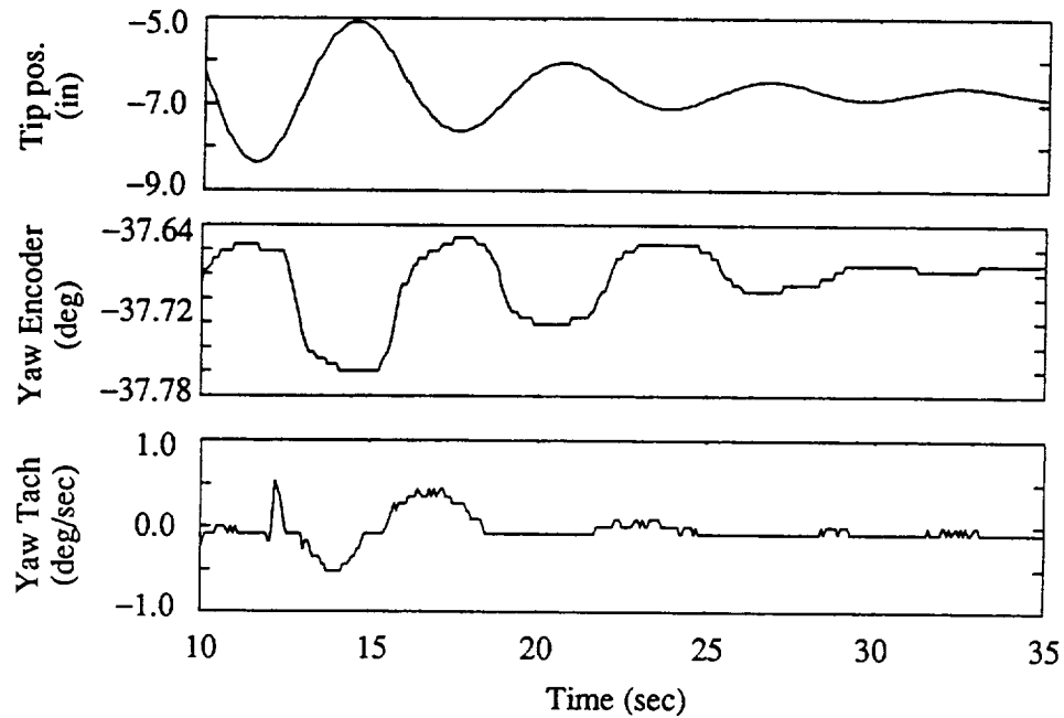
Figure 5.1.6 Typical RMS response and sensor outputs - \theta = 30^\circ .
