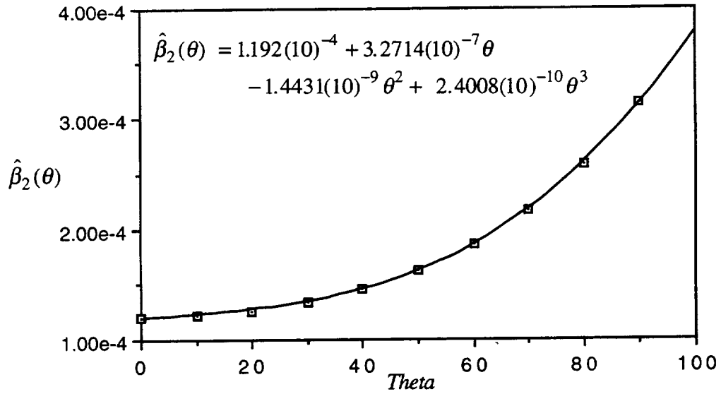
Figure 3.5.3 Identified Polynomial \hat{\beta}_2(\theta)
