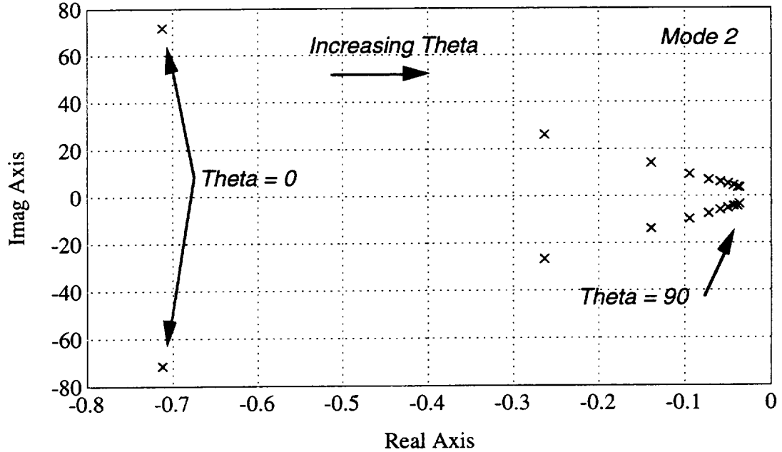
Figure 2.5.2 Second Mode poles as Function of Theta
