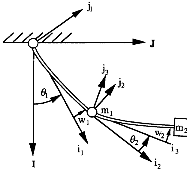
Figure 2.1 Flexible Manipulator
