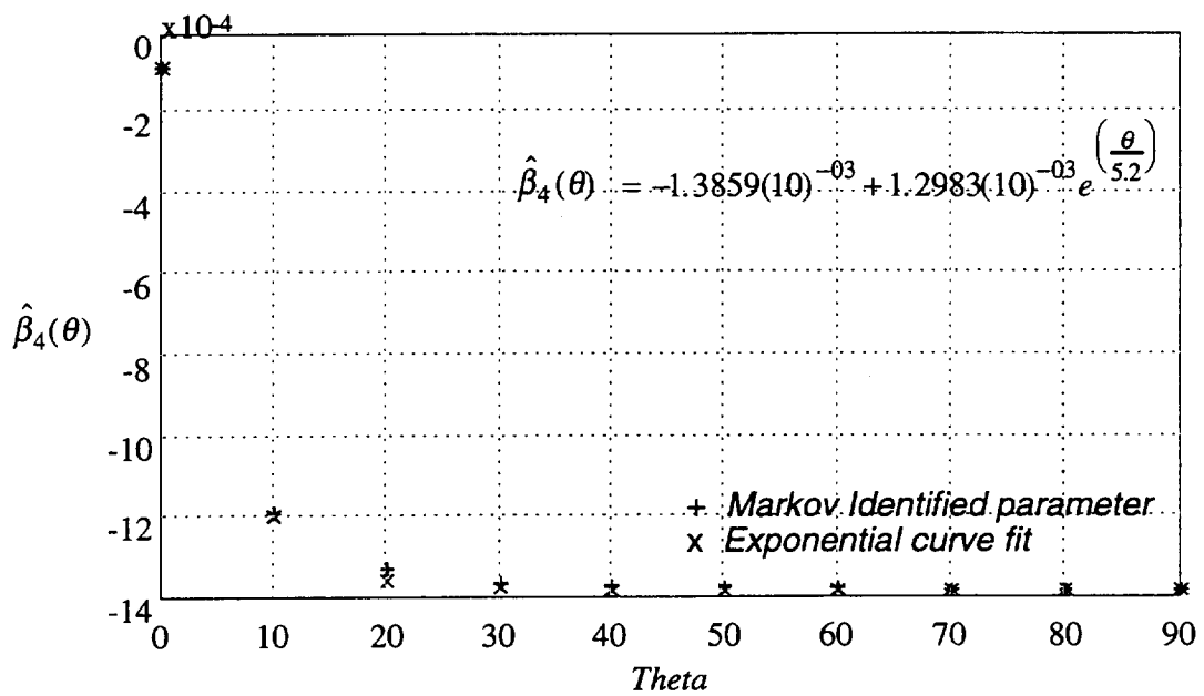
Figure 3.5.11 Identified Exponential Function \hat{\beta}_4(\theta) - p = 4
