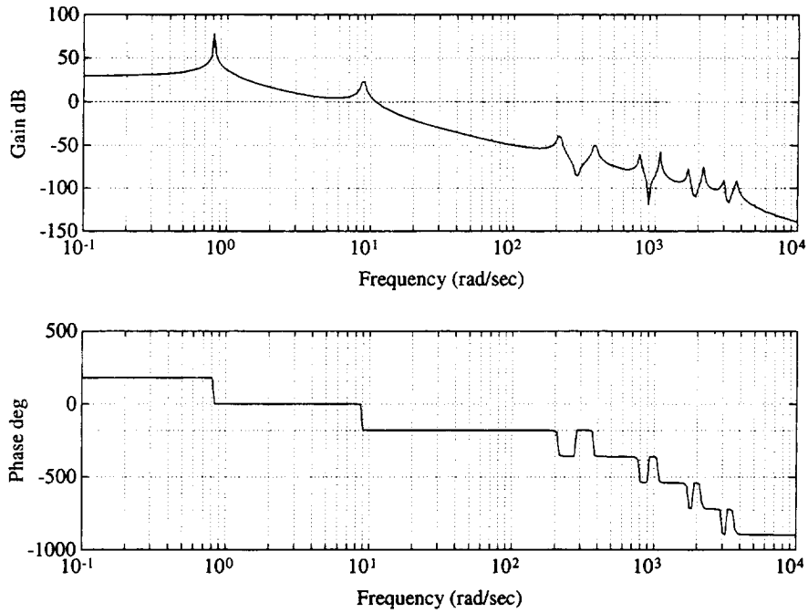
Figure 4.6.2 Bode Response of Nominal Plant Model G_n(s) at 50^\circ .
