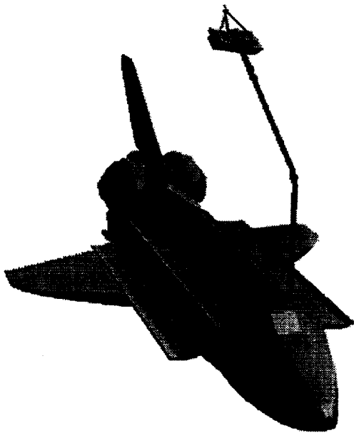
Figure 5.1.4 SRMS Configuration \theta = 60^\circ
