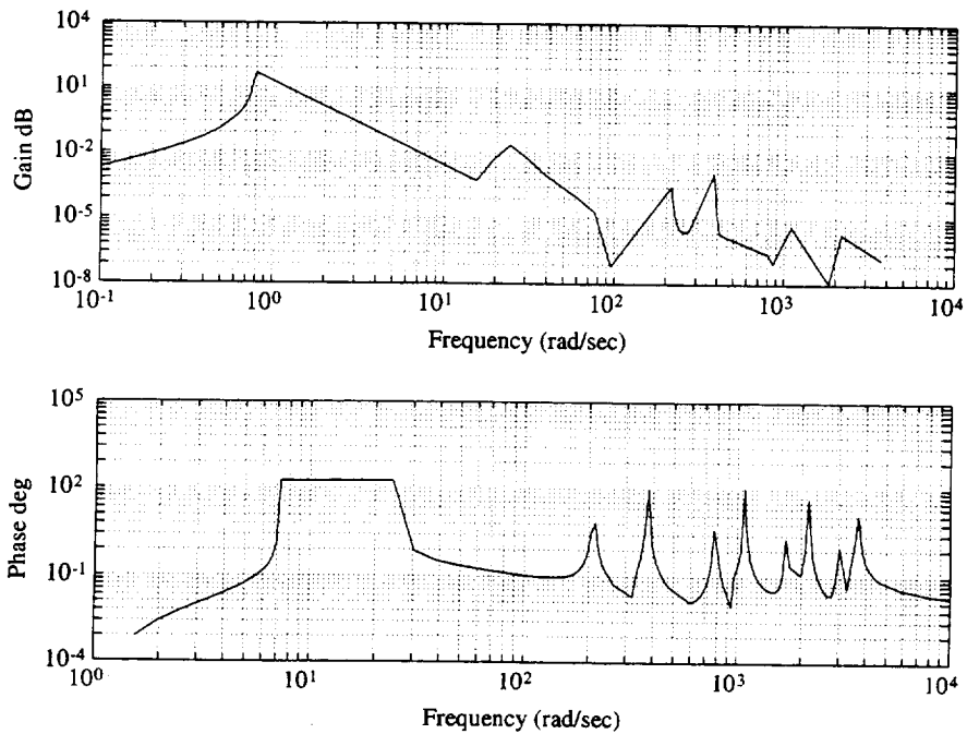
Figure 4.6.3 Maximum Bound on the Additive Model Error E_a(j\omega)
