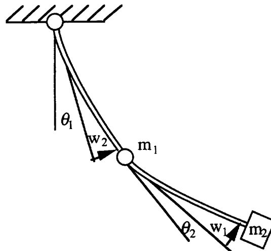
Figure 3.1 Two Link Model used for System Identification
