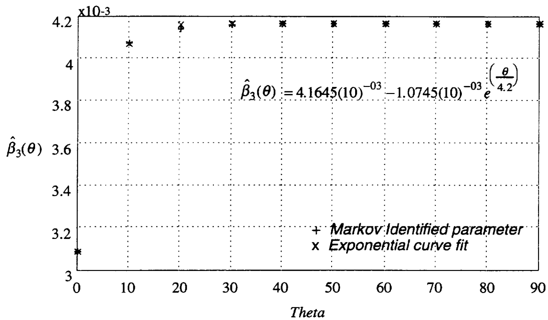
Figure 3.5.9 Identified Exponential Function \hat{\beta}_3(\theta) - p = 4
