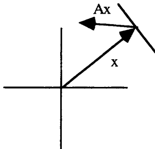
Figure A.1 Geometric Interpretation of \bar{A} + \bar{A}^T < 0
