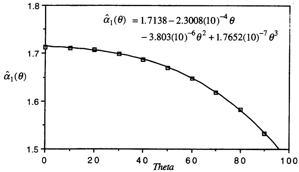
Figure 3.5.2 Identified Polynomial \hat{\alpha}_1(\theta) as Function of Theta
