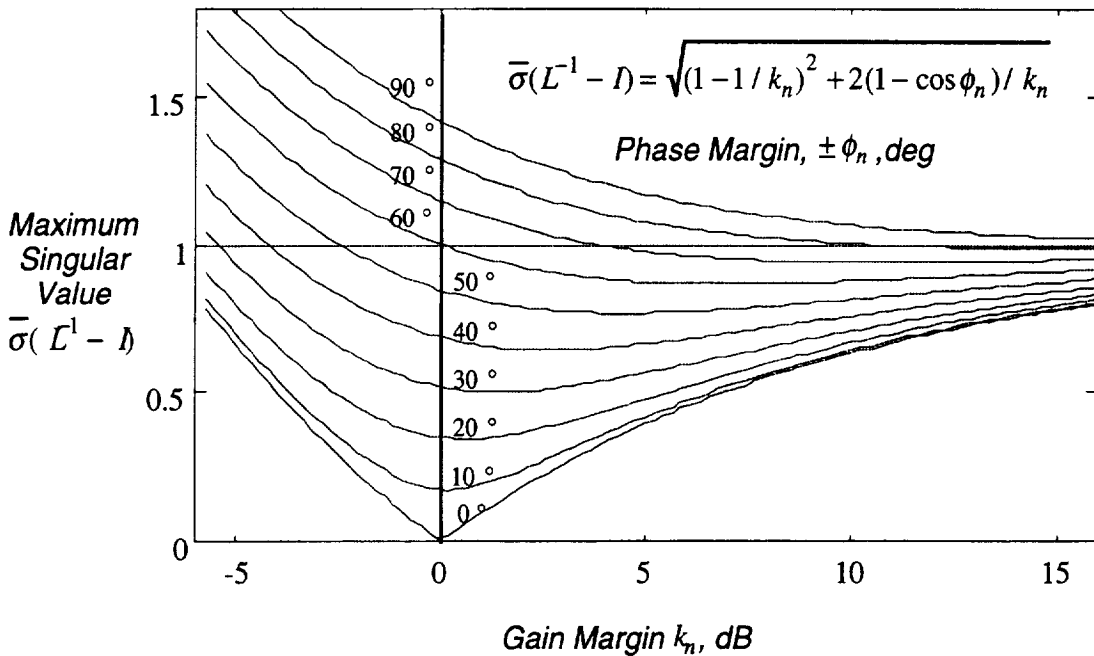
Figure 4.3.4 Universal Diagram for Gain-Phase Margin Evaluation
