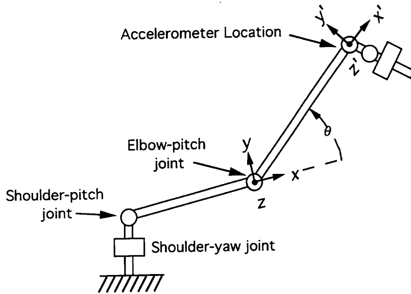
Figure 2.2.1 Six Degree of Freedom Manipulator
