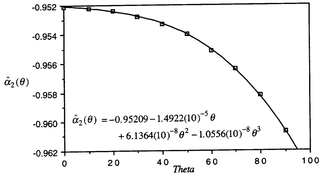
Figure 3.5.4 Identified Polynomial \hat{\alpha}_2(\theta)
