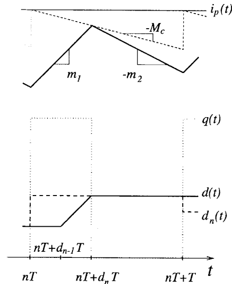
Fig. 9. Inductor-current waveforms for constant-frequency current-mode control, with relationships among q(t) , d(t) , d_n(t) , i_L(t) , and i_p(t) .
