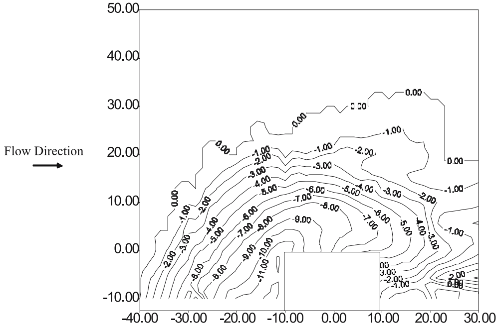
Figure 3. Contours of scour hole in cm around vertical abutment at t = 150 min.
