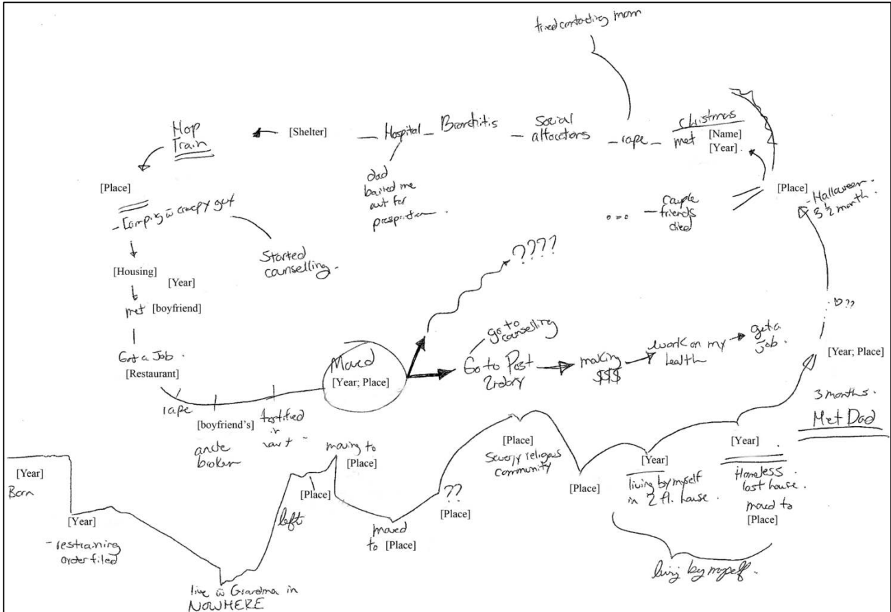
Figure 2. Continuous-line Timeline.
