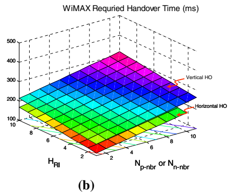
Fig. 11 The required handover time for WLAN and WiMAX. a WLAN. b WiMAX
