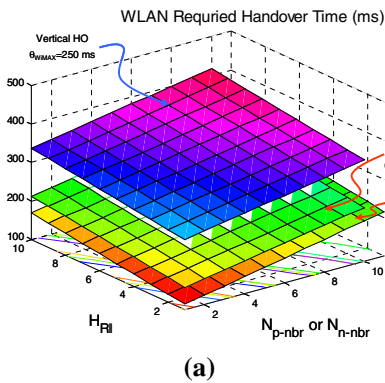
Fig. 11 The required handover time for WLAN and WiMAX. a WLAN. b WiMAX
