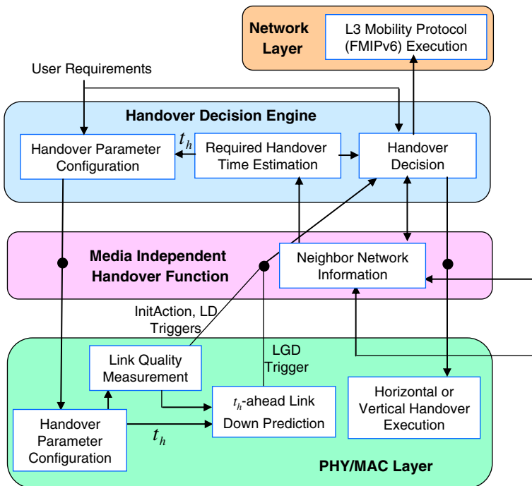
Fig. 2 The proposed predictive handover architecture based on the neighbor network information
