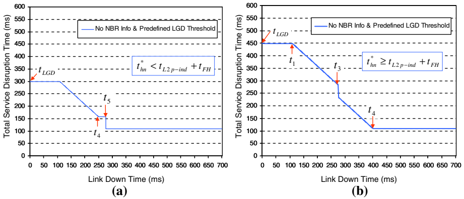
Fig. 13 The total service disruption time. a t_{hm}^* < t_{L2-ind} + t_{FH} . b t_{hm}^* \geq t_{L2-ind} + t_{FH}
