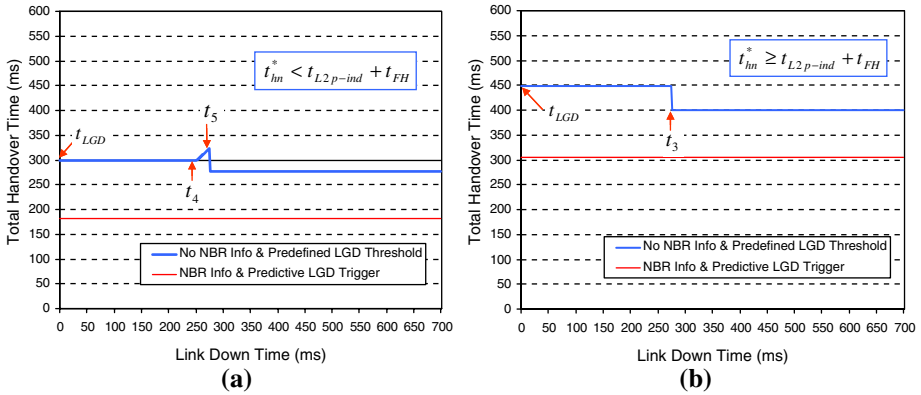
Fig. 12 The total handover time. a t_{hm}^* < t_{L2-ind} + t_{FH} . b t_{hm}^* \geq t_{L2-ind} + t_{FH}
