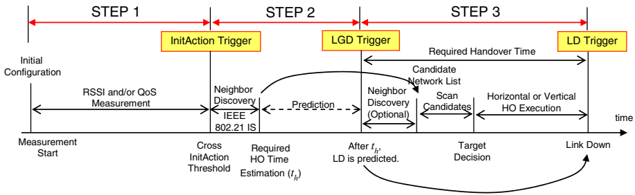
Fig. 3 Predictive handover time sequence
