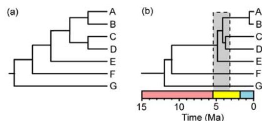
Fig. 1. Relationship between a phylogenetic tree (a) showing only the branching order of seven species, and the corresponding time-tree (b) showing both branching order and times of divergence. Colored horizontal panels represent geologic periods, and the gray vertical bar represents a climatic or geologic event.
