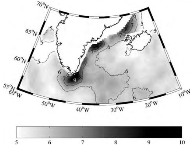
FIG. 5. The standard deviation of the winter (DJF) 10-m wind speed field ( \text{m s}^{-1} ) from the QuikSCAT dataset (1999–2004).
