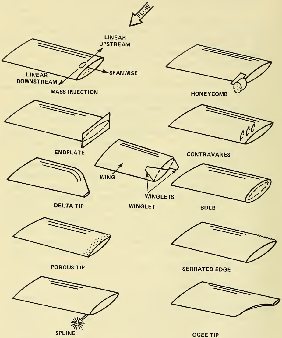
Figure 4 - Illustration of Schemes for Alleviating Tip Vortex
