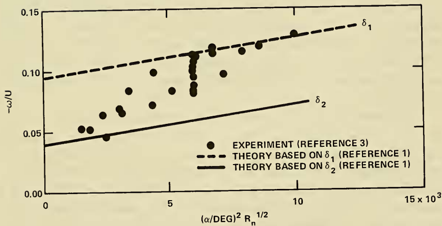
Figure 3 - Variation of Tip-Vortex Core Axial Velocity w_0 with Reynolds Number R_n
