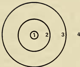
Figure 2 - Proposed Spatial Distribution of Vortex Structure: 1 - Viscous Inner Region; 2 - Smoothed-Out Spiral, Velocity Distribution Essentially Inviscid; 3 - Tightly Wound Spiral; and 4 - Unrolled Portion of Vortex Sheet
