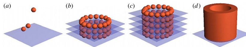
Figure 13. Layer-by-layer deposition. (a) A sheet of biocompatible hydrogel is printed, and the building blocks are embedded into the hydrogel. (b) and (c) The alternate deposition of layers of hydrogel and building blocks is pursued according to the predefined blueprint of the desired 3D structure (here, a tubular construct). (d) Fusion of the building blocks and removal of the hydrogel result in a hollow tube after a few days.
