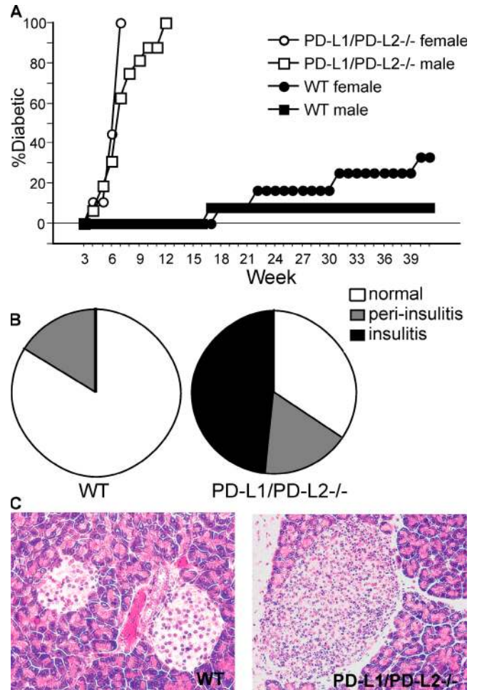
Figure 3. Loss of PD-L1 and PD-L2 results in the rapid onset of diabetes and the early onset of insulitis. (A) PD-L1/PD-L2 -/- N4 mice on the autoimmune diabetes-prone NOD background were monitored for the development of hyperglycemia. Animals were scored as diabetic upon blood glucose readings of \geq 250 mg/dL, and diabetes was confirmed by three consecutive positive reads. Both female PD-L1/PD-L2 -/- NOD mice ( n = 9 ) and male PD-L1/PD-L2 -/- NOD mice ( n = 16 ) develop autoimmune diabetes significantly ( P < 0.0001 ; unpaired t test) faster than WT littermate controls (females, n = 12 ; males, n = 13 ). (B) PD-L1/PD-L2 -/- and WT N5 NOD littermates were analyzed for early and late signs of immune cell infiltration of the pancreatic islets by histology. Pancreata from PD-L1/PD-L2 -/- and WT NOD littermates ranging in age from 27 to 50 d were evaluated histologically. Islets were scored as normal, peri-insulitic, or insulitic, and the percentage of total islets in each category was averaged for each group. Three of nine PD-L1/PD-L2 -/- mice were hyperglycemic, and all 10 WT animals were euglycemic at the time of killing. (C) Representative islets from WT (left; scored as normal) and PD-L1/PD-L2 -/- (right; scored as insulitic) pancreas are shown. Islets pictured are from 50-d-old littermate females with normal blood glucose readings immediately before killing.
