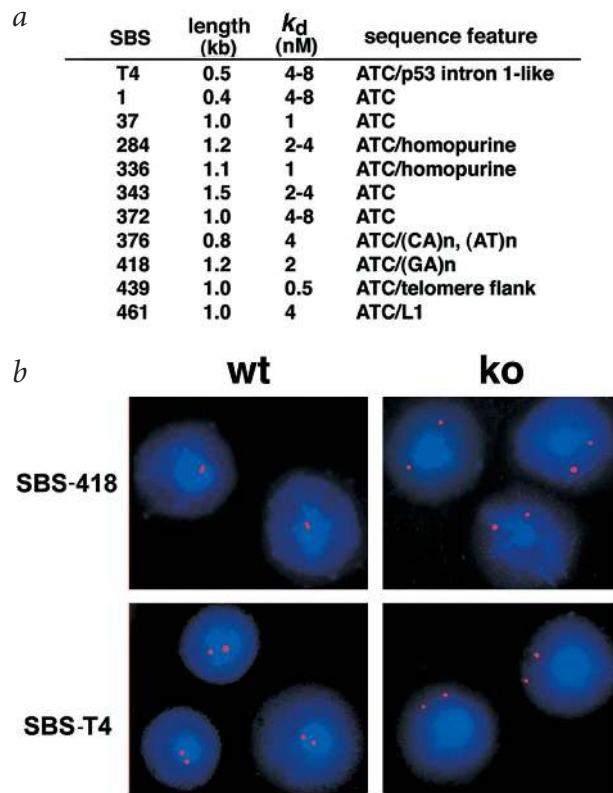
Fig. 4 Isolation and characterization of individual genomic sequences that bind to SATB1 in vivo in mouse thymocytes. a , Individual sequences were cloned from an in vivo crosslinked chromatin fraction specifically immunoprecipitated by antibody against SATB1 according to a published method 35 . Dissociation constant ( k_d ) values were determined as described 32 and the sequence characteristics are shown. All sequences have the ATC sequence context. b , Amplified FISH data is shown using SBS-418 and SBS-T4 as probes for in situ prepared DNA halos from wild-type (wt) and Satb1 -knockout (ko) thymocytes as described for Figure 2. Similar analyses were done for the four additional SBSs, and identical results were obtained (data not shown).
