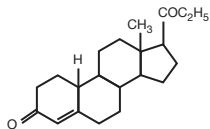
19-norprogesterone
