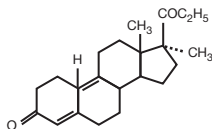
Promegestone (R5020)
