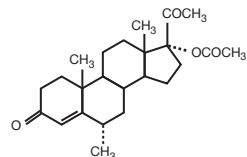
Medroxyprogesterone acetate
