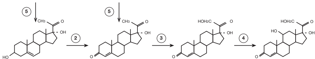
17 \alpha -Hydroxypregnenolone
