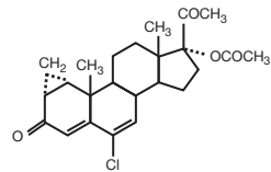
Cyproterone acetate
