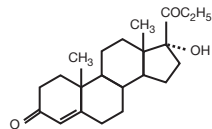
17a-hydroxyprogesterone
