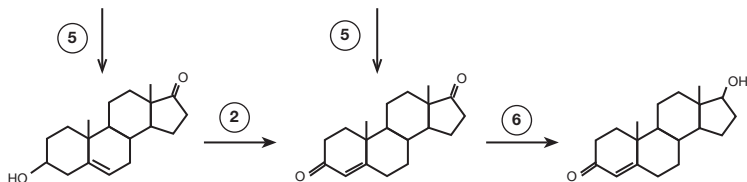
Dehydroepiandrosterone
