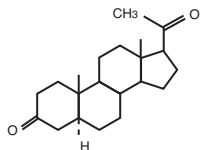
5 \alpha -Dihydroprogesterone
