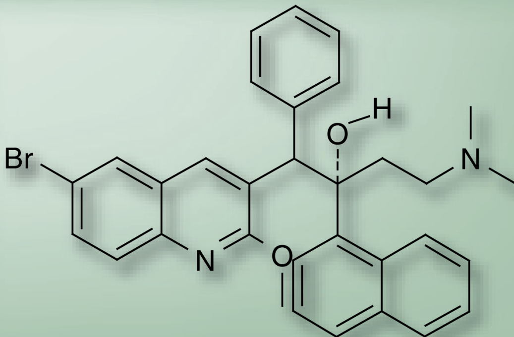
Figure 1. TMC207 (R207910).
