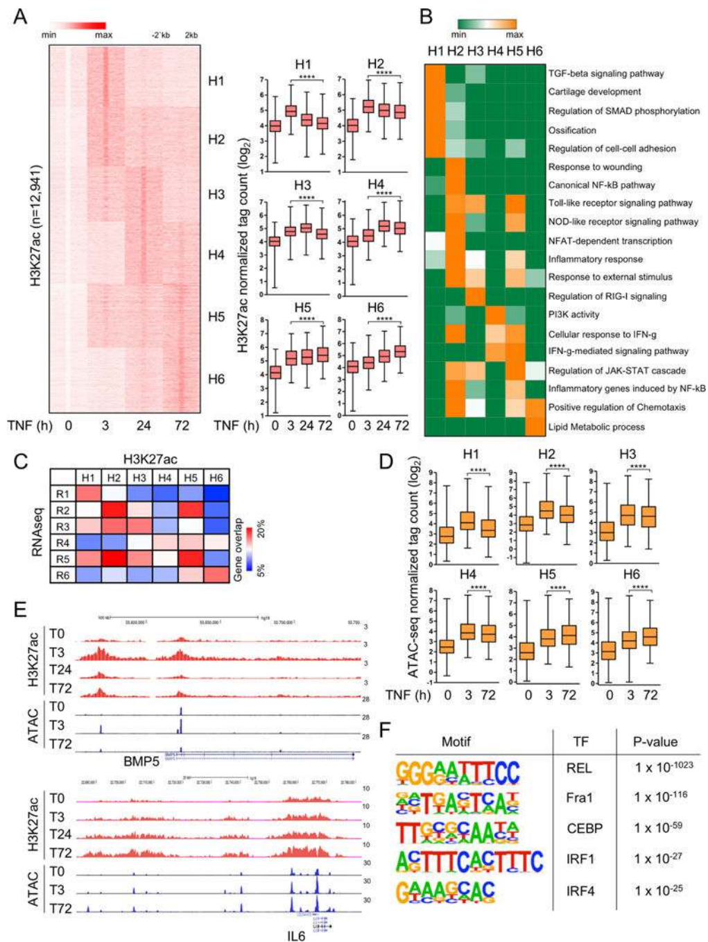
Figure 3. Epigenomic landscape changes in FLS after TNF exposure. (A) Genome-wide H3K27ac ChIP-seq analysis (two biological replicates from independent patients with RA) of differentially induced peaks at each TNF-stimulated time points (3, 24 and 72 hours). The left panel depicts K-means clustering of 12 941 peaks (one per row) that were induced more than fourfold by TNF ( p < 0.0001 ) into six clusters (H1–H6); expression is presented relative to the maximum (set as 1). Box graphs represent H3K27ac ChIP-seq normalised tag densities (log 2 ) at enhancers of a given cluster under the indicated conditions (right).
