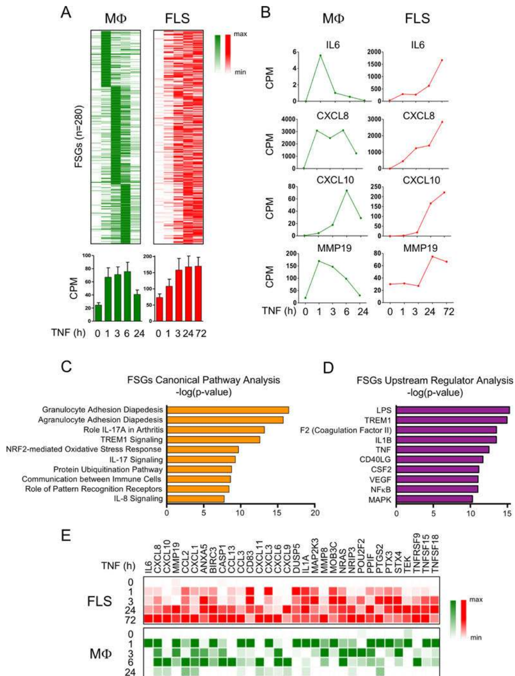
Figure 1. Genes that are transiently induced by TNF in macrophages exhibit sustained expression in FLS. (A) Kinetic analysis of TNF-induced mRNA transcripts whose expression is transient in macrophages but sustained in FLS. RNA-seq analysis was performed in a time course of TNF stimulation (10 ng/mL) using macrophages (three replicates from independent blood donors) and FLS (two replicates from independent patients with RA). Two hundred and eighty genes (FSGs) transiently expressed in macrophages but sustained in FLS are displayed on a heatmap (upper panels). Bar graphs (lower panels) represent CPM values for
