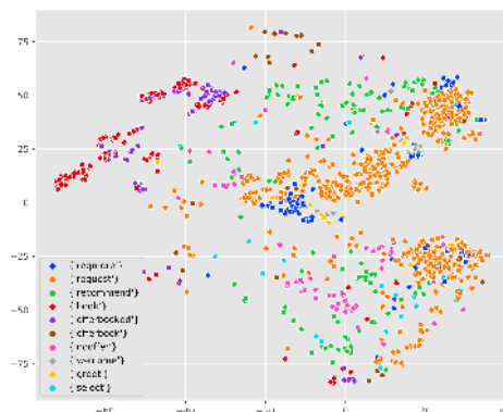
(b) TOD-BERT-mlm
