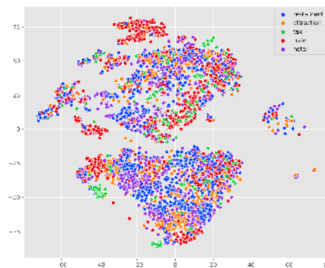
(b) TOD-BERT-mlm
