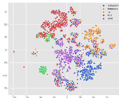
(c) TOD-BERT-jnt
