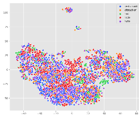
(a) BERT
