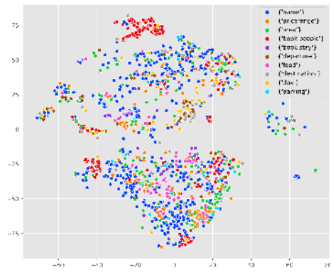
(b) TOD-BERT-mlm
