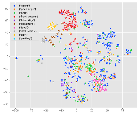
(c) TOD-BERT-jnt
