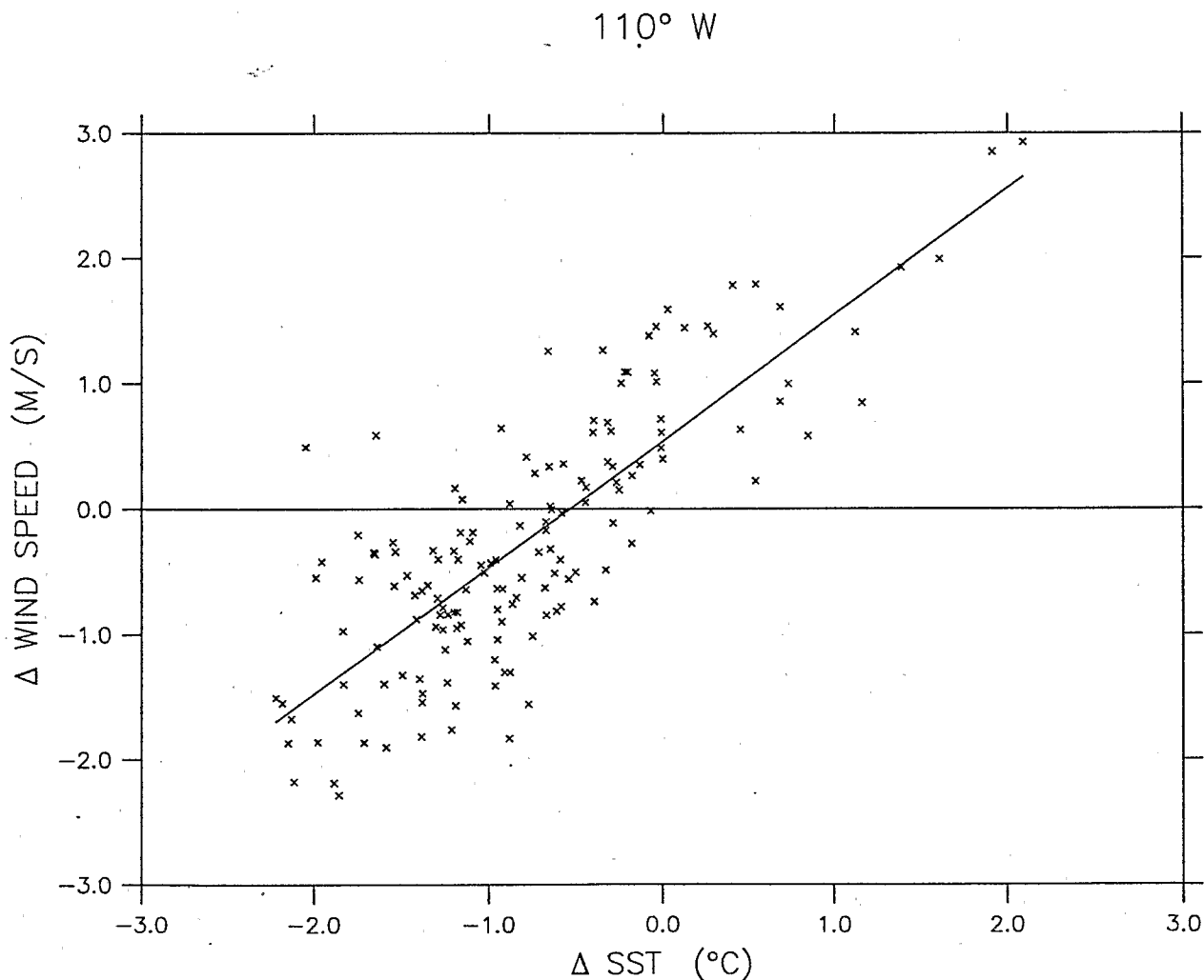
FIG. 4. Scatter plot of the change in wind speed along 110°W between the equator and 2°S ( \Delta S) vs. the change in temperature ( \Delta T) between these two latitudes for daily average measurements from July to November 1988. The correlation coefficient between these variables is 0.63.
