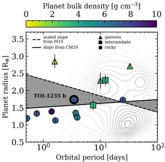
Figure 8. Period–radius diagram for small planets orbiting M dwarfs with precise RV masses, including TOI-1235 b (thick circle). The dashed and solid lines depict the locations of the radius valley around low-mass stars from model predictions of thermally driven atmospheric mass loss and from gas-poor terrestrial planet formation, respectively. The shaded regions highlight where the predictions of planetary bulk compositions are discrepant between the two models. Contours represent the planetary occurrence rates around low-mass stars (CM19). Planet marker shapes depict the planet’s compositional disposition as either rocky (circles), gaseous (triangles), or intermediate (squares). Marker colors indicate the planet’s bulk density.
