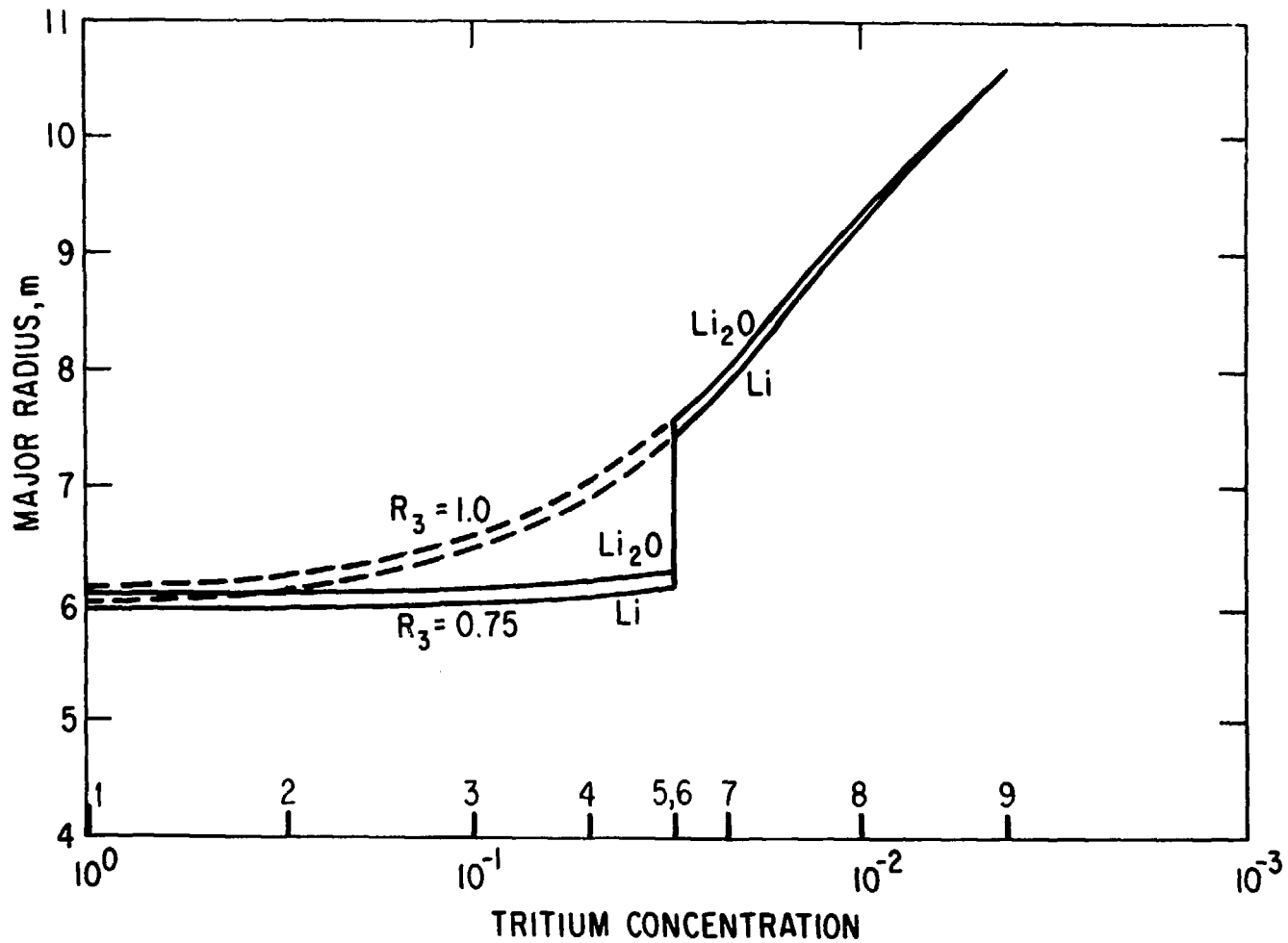
Fig. 10. Major radius as a function of tritium concentration for fixed thermal power and first-wall heat load.
