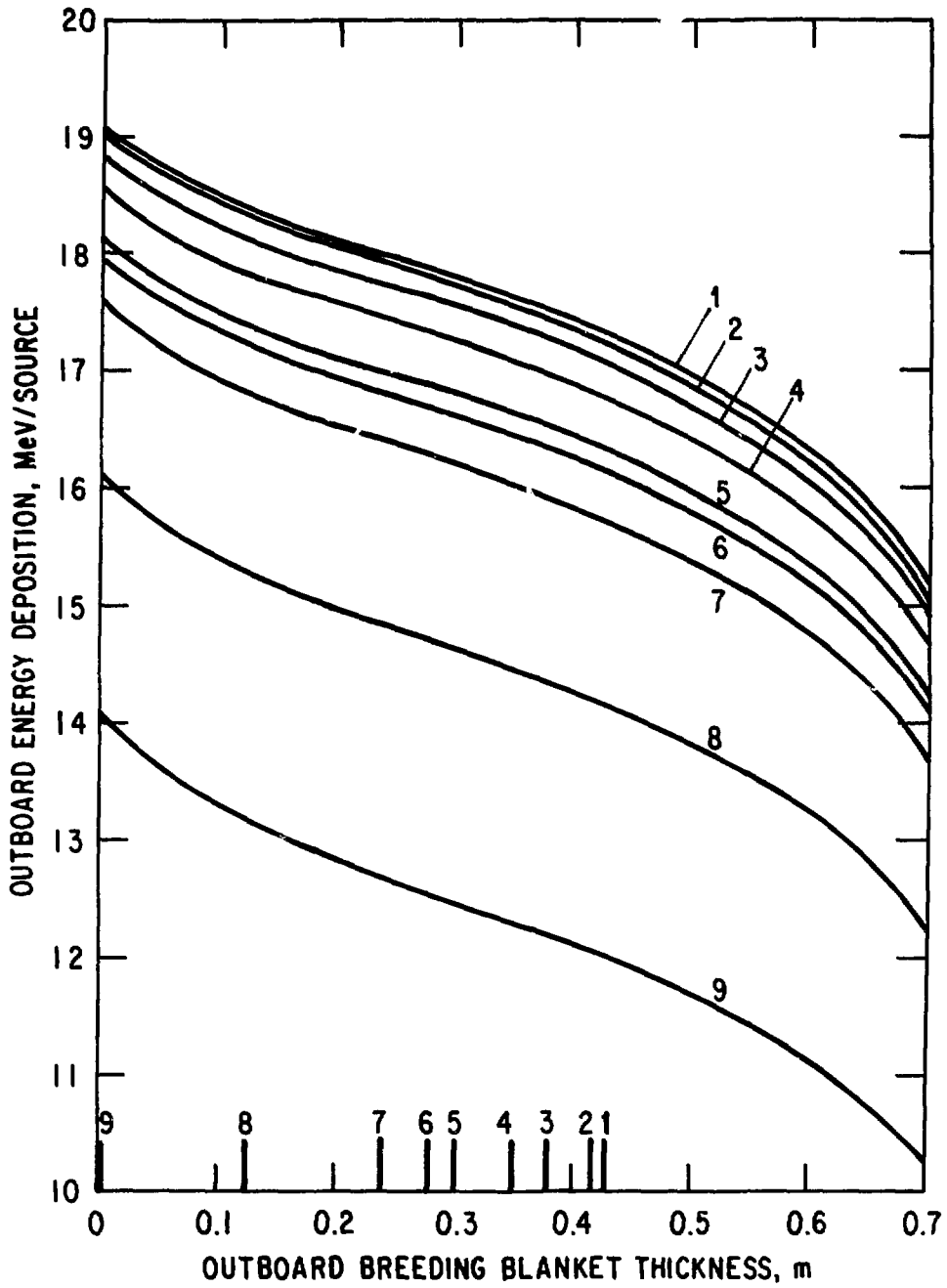
Fig. 7. Outboard energy deposition - liquid lithium breeder.
