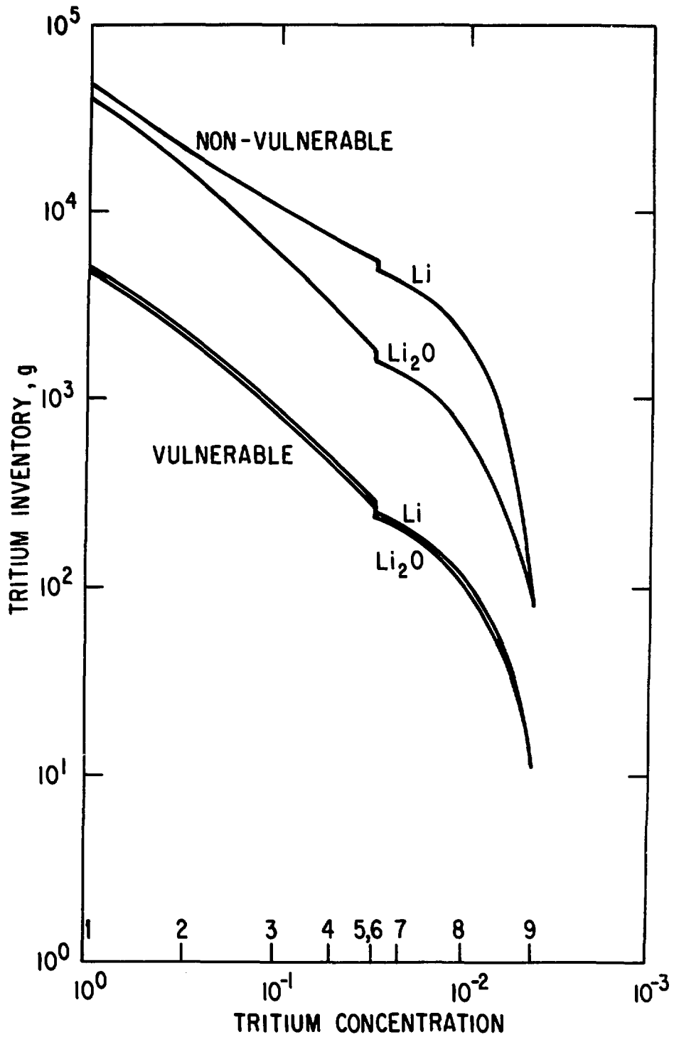
Fig. 13. Tritium inventories.
