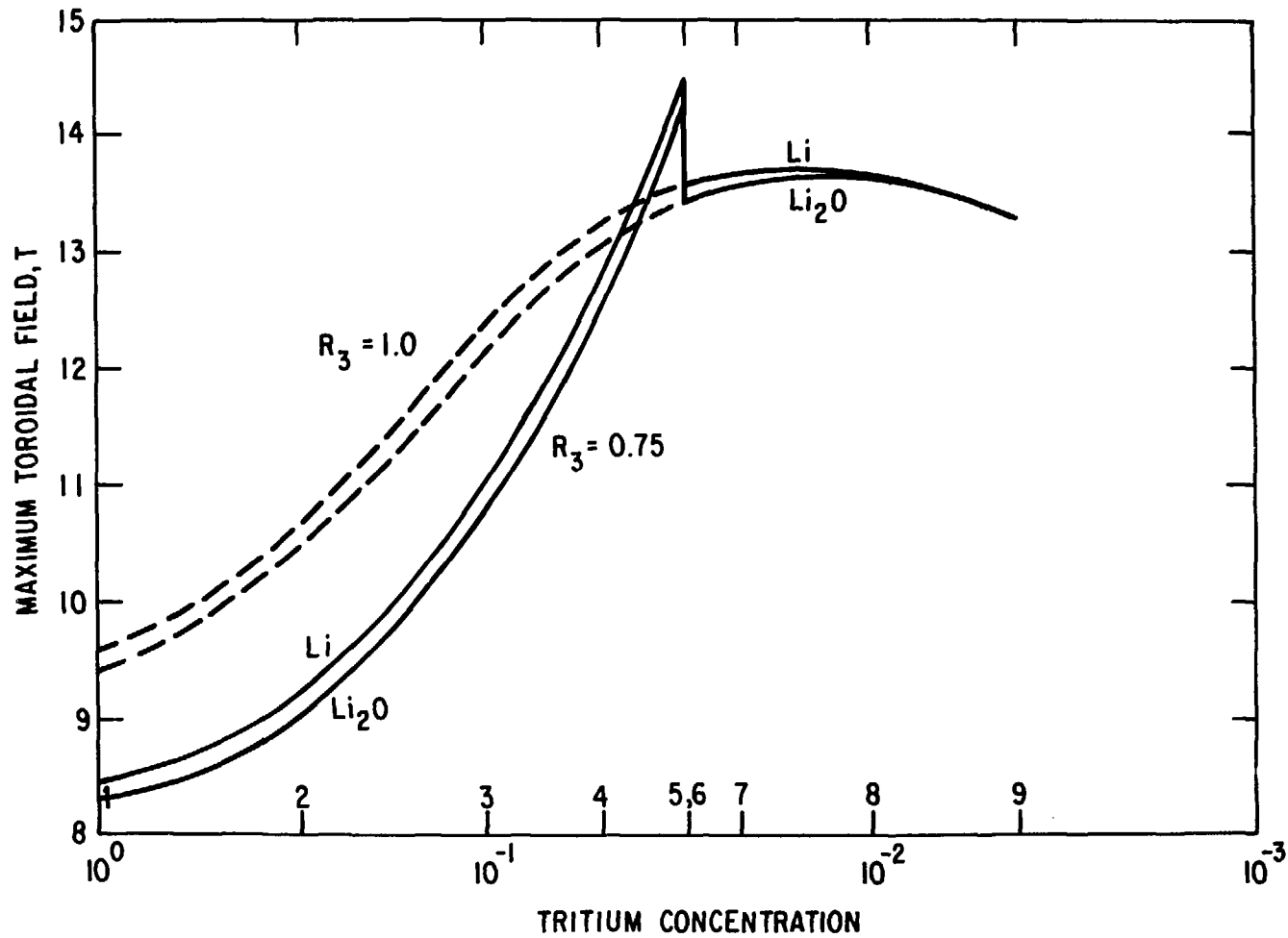
Fig. 11. Peak toroidal field as a function of tritium concentration for fixed thermal power and fixed wall heat load.
