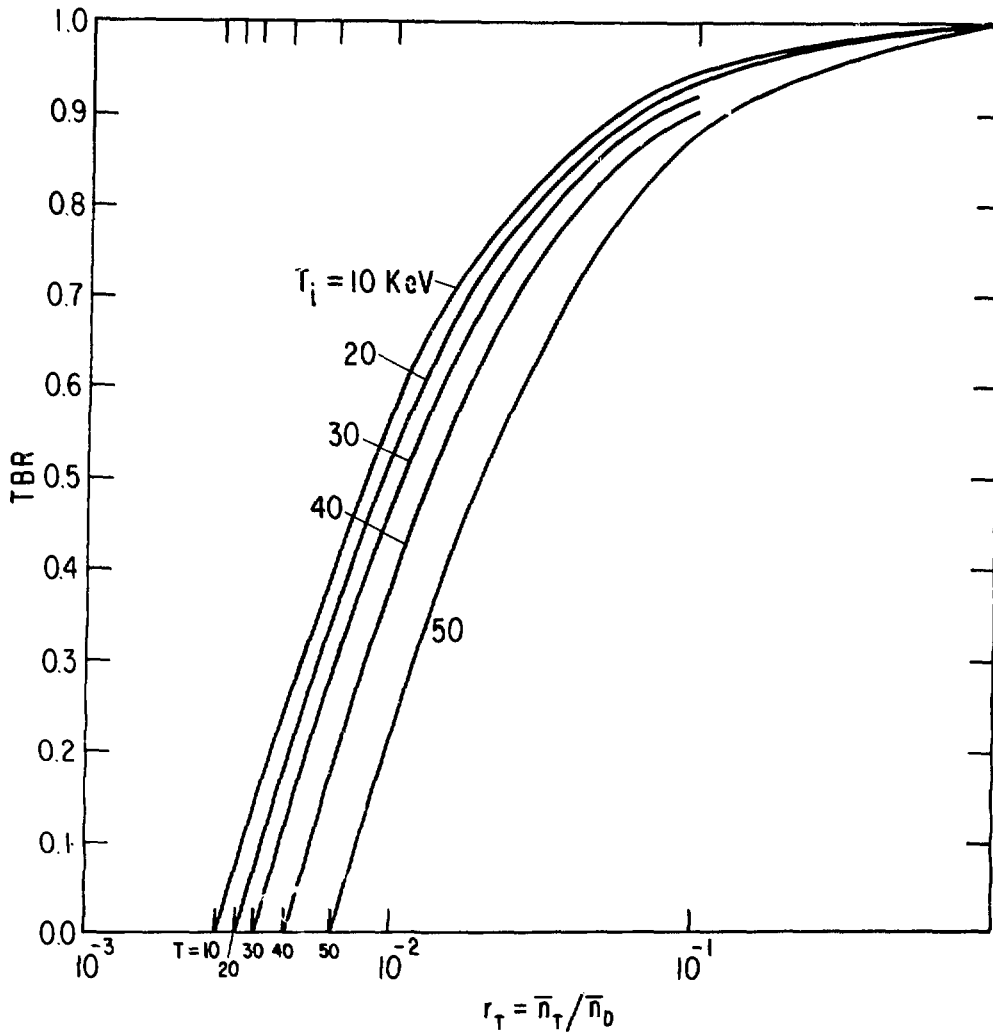
Fig. 1. Approximate expression for the tritium breeding ratio as a function of tritium concentration.
