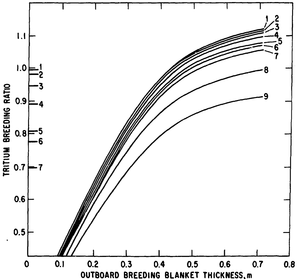
Fig. 5. Tritium breeding ratio obtained with a given outboard breeding blanket thickness - liquid lithium breeder.
