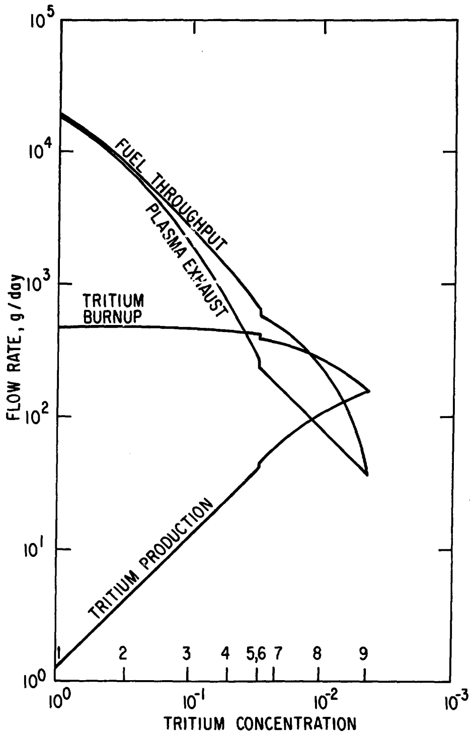
Fig. 12. Rates of tritium burnup, production, exhaust, and fueling.
