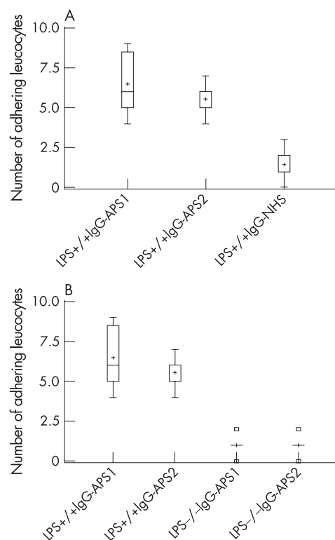
Figure 2 Effect of antiphospholipid (aPL) antibodies on adhesion of leucocytes to endothelium in lipopolysaccharide (LPS) non-responsive mice. LPS +/+ and LPS -/- mice in groups of 7–10 were injected with IgG from patients with antiphospholipid syndrome (IgG-APS) or with IgG from normal human serum (IgG-NHS) 0 and 48 h later (as described in the Methods section). Adhesion of leucocytes (number of white blood cells (WBC)) to endothelium in post-capillary venules of the cremaster muscle was measured as described in the Methods section. The results are expressed as the median (range) SD of the number of adhering WBC. (A) The median number of adhering WBC in LPS +/+ mice treated with IgG-APS was significantly different from the median number of adhering WBC in LPS +/+ mice treated with IgG-NHS (for IgG-APS-1 and IgG-APS-2). (B) The median number of adhering WBC in LPS -/- mice treated with IgG-APS was significantly different from the median number of adhering WBC in LPS +/+ mice treated with IgG-APS (for IgG-APS-1 and IgG-APS-2). Squares indicate outliers. Plus signs indicate mean values.
