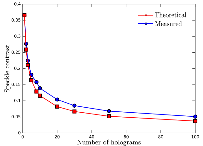
Fig. 7. Evolution of the speckle contrast with the number of illuminations in TDM.
