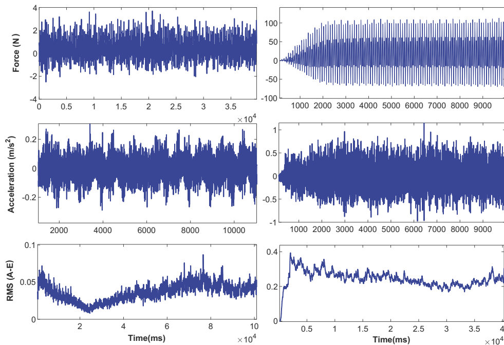
Fig. 5 Sensors measurement for the first cycle (right) and last cycle (left) of machining
