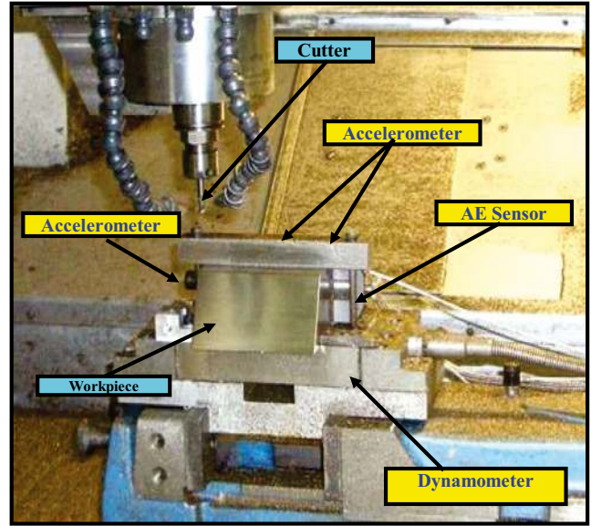
Fig. 4 Experimental setup
