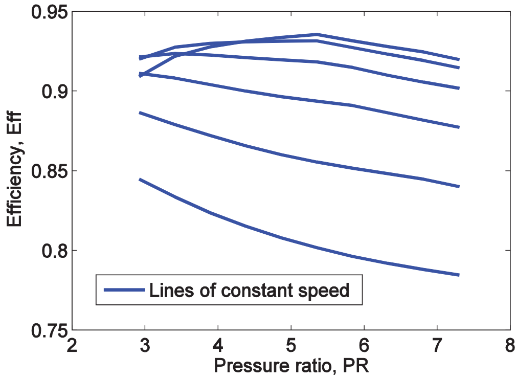
Figure 8.—Sample turbine map (efficiency vs. pressure ratio).
