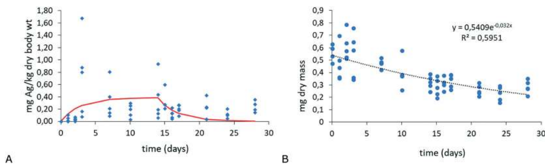
Fig. 3 A: Ag uptake and elimination in E. crypticus exposed to Ag 2 S-NMs (20 nm, 2.5 mg Ag per kg dry soil) (x-axis: days; y-axis: mg kg -1 ). B: Mass over time of animals during the uptake and elimination kinetics test (x-axis: days; y-axis: mg dry mass).
