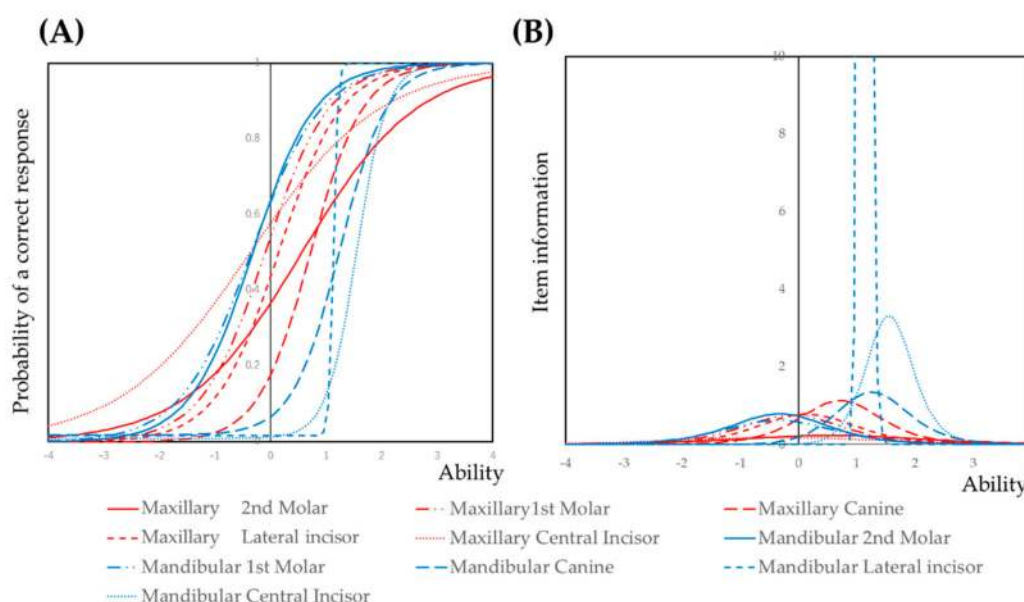
Figure 1. Item response curves and item information curves for the prevalence of dental caries. (A) Item response curve; (B) item information curve. In item response theory (IRT) analysis, the discriminatory power of an item is presented by the steepness of the curve at its inflection point and height of the item information curve. A steep curve and high item information indicate a distinction between respondents with low ability levels versus those with high ability levels. The item response curve and item information curve located in the forward direction indicated that subjects with high ability have a probability of a correct response. The item response curve and item information curve located in the backward direction indicate that even subjects with low ability can respond correctly. Susceptibility for dental caries was different between tooth types. The maxillary central incisor was found to often have dental caries. By contrast, the item response curve of the mandibular lateral incisor was steep and located in the forward direction, and the item information curve was high. It indicated that the mandibular lateral incisor often did not have dental caries. If dental caries was detected in the mandibular lateral incisor, most of the teeth were found to have dental caries in the primary dentition.
