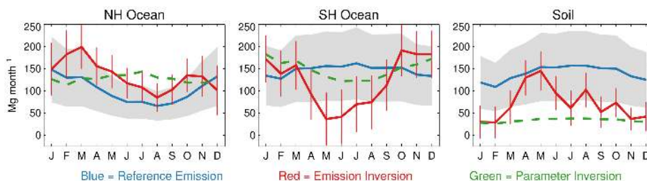
Figure 5. Monthly emissions for the three seasonal sources (NH ocean, SH ocean, and soil) from the reference simulation (blue solid lines), emission inversion (red solid lines), and parameter inversion (green dashed lines). The gray shaded regions and red error bars indicate 1\sigma uncertainties for the reference emissions and emission inversion, respectively.
