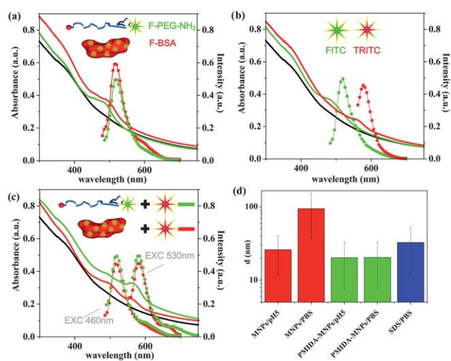
Fig. 4 (a) UV-visible spectra of non-functionalized FeO x -MNPs (black line), FeO x -MNPs conjugated with F-BSA (red line) and F-PEG-NH 2 (green line). The absorption band of fluorescein at 490 nm is evident in both cases. The dotted green lines are the corresponding fluorescence spectra. (b) UV-visible spectra of non-functionalized FeO x -MNPs (black line), FeO x -MNPs conjugated with FITC (green line) and TRITC (red line) with the relative fluorescence emission spectra (dotted lines). The absorption bands of fluorescein at 490 nm and of rhodamine at 560 nm are evident in both cases. (c) UV-visible (straight lines) and fluorescence (dotted lines, excitation at 460 nm or 530 nm) spectra of FeO x -MNPs after sequential functionalization with F-BSA and TRITC (red lines) or with F-PEG-NH 2 and TRITC (green lines). (d) Average size and relative standard deviation of FeO x -MNPs at pH 4 and in PBS solutions measured by DLS.
