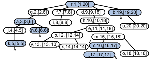
Figure 3: A Tree T with Preorder and Interval on Each Node
