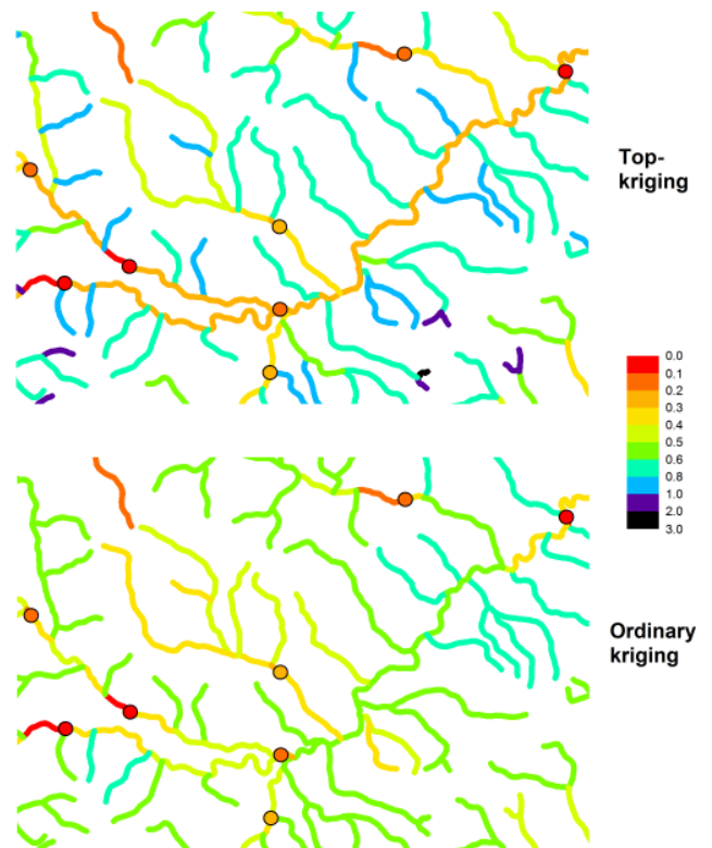
Fig. 9. Uncertainties of the normalised specific 100-year flood Q_{100N} from Top-kriging (top) and Ordinary Kriging (bottom), expressed as the coefficient of variation, colour coded on the stream network of the Mur region. Uncertainties of the measurements (i.e. values at the stream gauges) are shown as circles.
